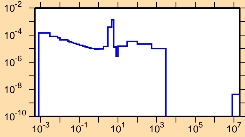
\sigma vs. E for ^{223}\text{At}(n,f)
