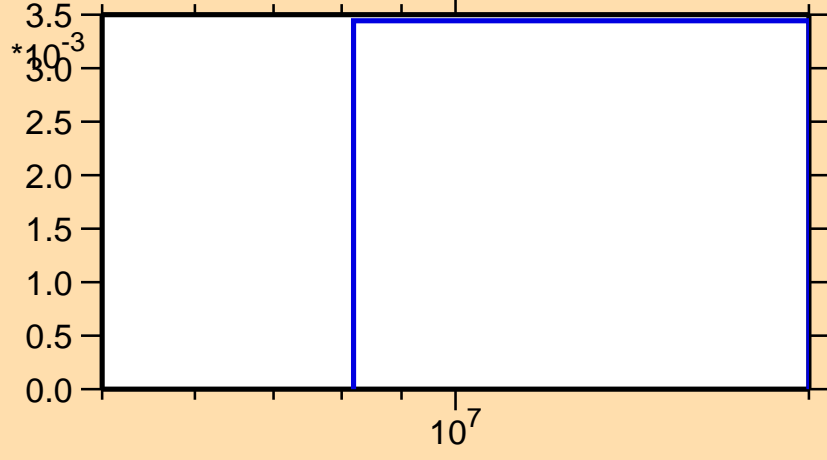
\sigma vs. E for ^{223}\text{At}(n,3n)
