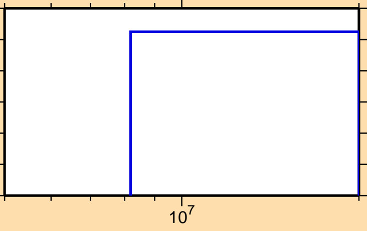
\sigma vs. E for ^{223}\text{At}(n,nt)
