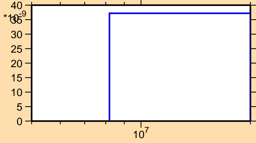
\sigma vs. E for ^{223}\text{At}(n,2np)
