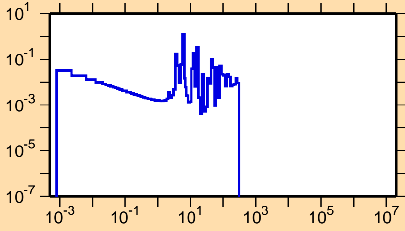
\sigma vs. E for ^{224}\text{At}(n,f)
