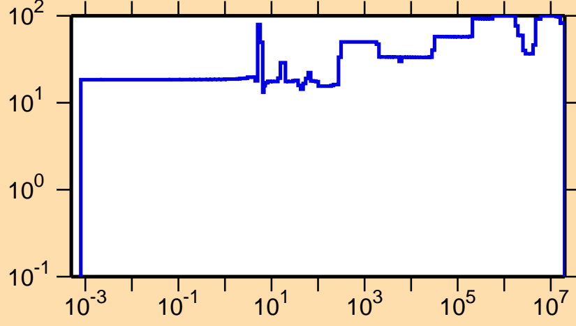
\Delta\sigma/\sigma vs. E for ^{224}\text{At}(n,el.)
