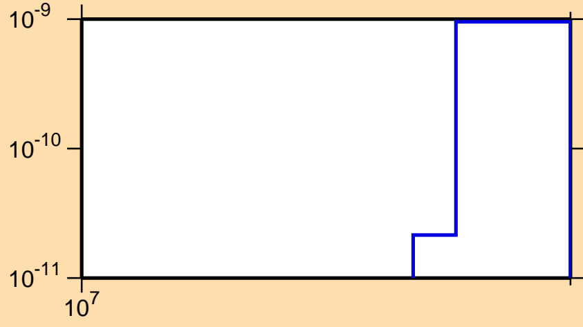
\sigma vs. E for ^{224}\text{At}(n,\text{He3})
