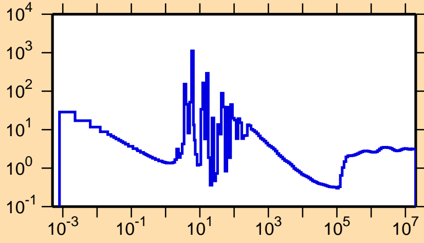
\sigma vs. E for ^{224}\text{At}(n,\text{nonel.})
