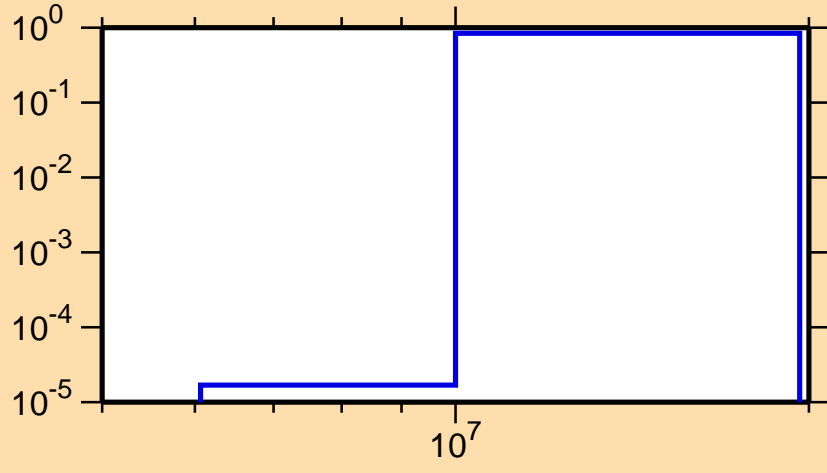
\sigma vs. E for ^{224}\text{At}(n,np)
