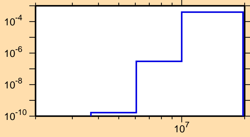
\sigma vs. E for ^{224}\text{At}(n,n\alpha)
