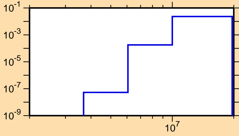
\sigma vs. E for ^{224}\text{At}(n,p)
