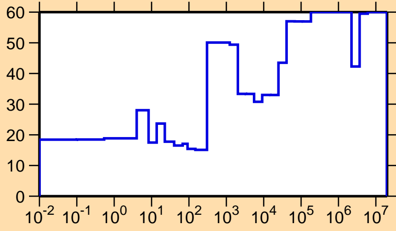
\Delta\sigma/\sigma vs. E for ^{224}\text{At}(n,el.)
