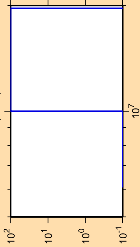
\Delta\sigma/\sigma vs. E for ^{224}\text{At}(n,nd)
