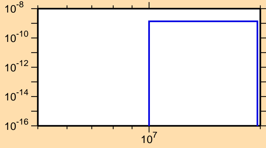
\sigma vs. E for ^{224}\text{At}(n,nd)
