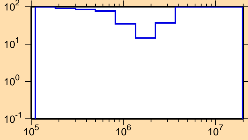
\Delta\sigma/\sigma vs. E for ^{224}\text{At}(n, ncont.)
