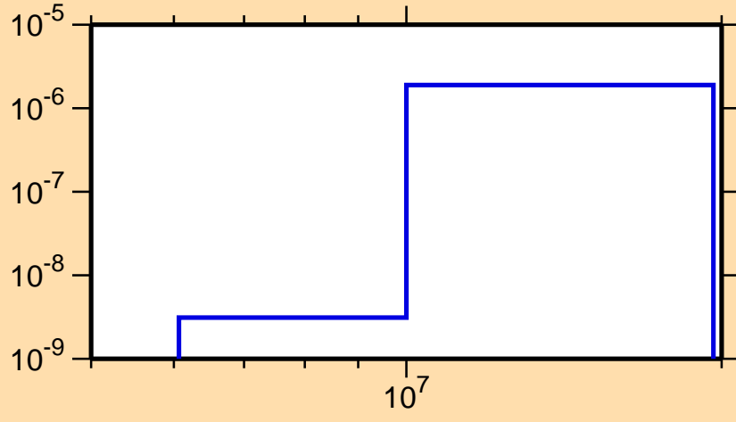
\sigma vs. E for ^{224}\text{At}(n,2n\alpha)
