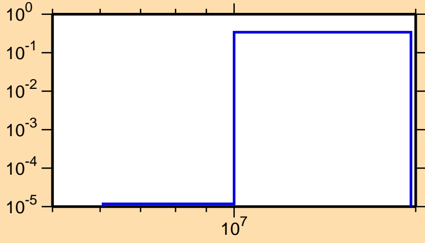
\sigma vs. E for ^{224}\text{At}(n,d)
