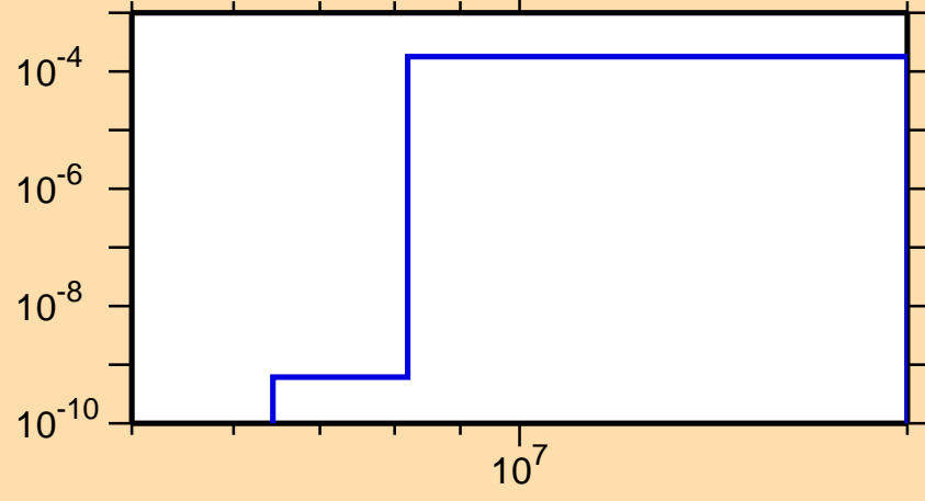
\sigma vs. E for ^{224}\text{At}(n,t)
