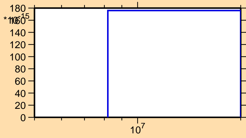
\sigma vs. E for ^{224}\text{At}(\text{mt } 42)
