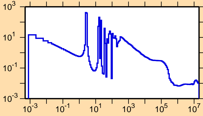
\sigma vs. E for ^{225}\text{At}(n,\gamma)
