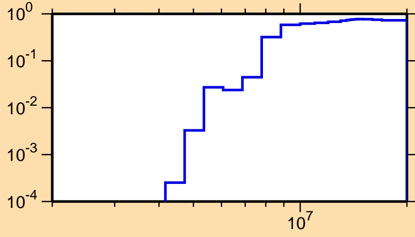
\sigma vs. E for ^{225}\text{At}(n,n\alpha)
