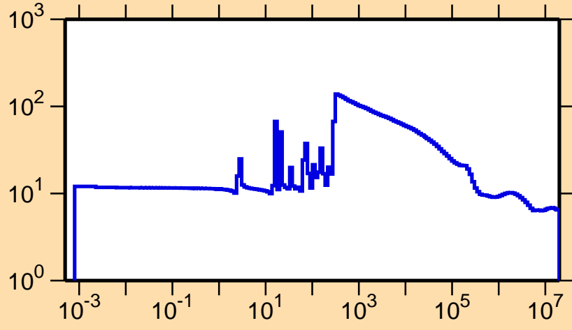
\sigma vs. E for ^{225}\text{At}(n,\text{el.})
