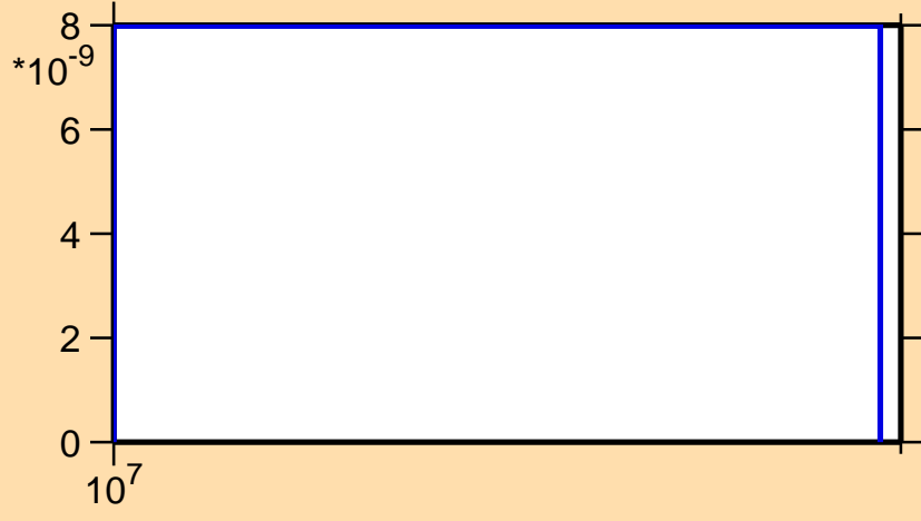
\sigma vs. E for ^{225}\text{At}(n,2np)
