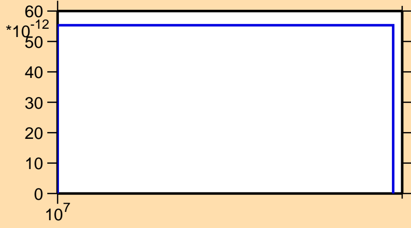
\sigma vs. E for ^{225}\text{At} (mt 11)
