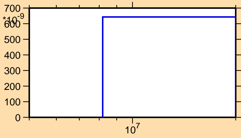
\sigma vs. E for ^{225}\text{At}(n,\text{nd})
