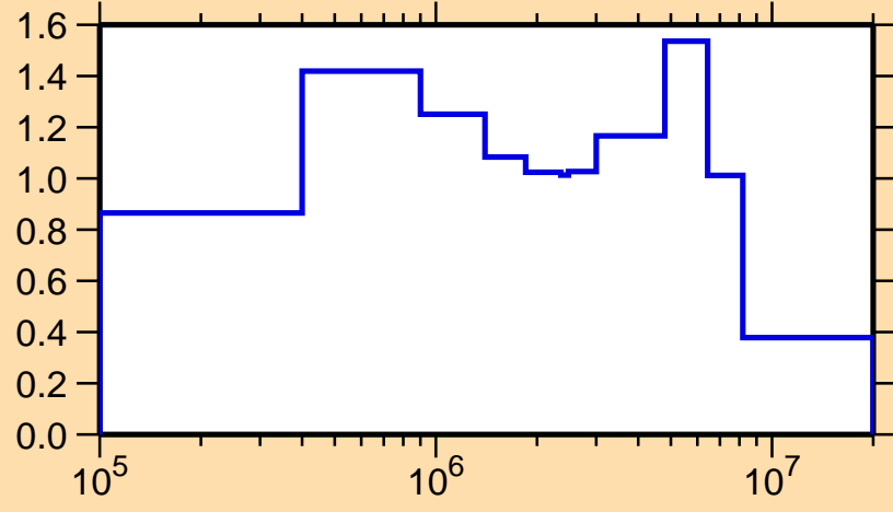
\sigma vs. E for ^{225}\text{At}(n,n\text{cont.})
