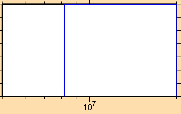
\sigma vs. E for ^{225}\text{At}(n,2np)
