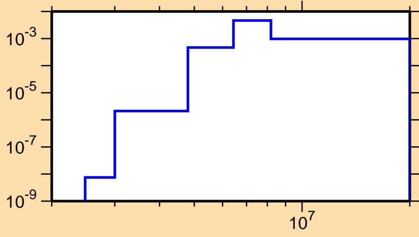
\sigma vs. E for ^{225}\text{At}(n,\alpha)
