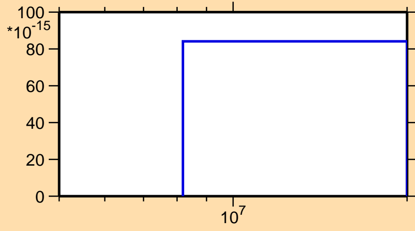
\sigma vs. E for ^{225}\text{At} (mt 42)
