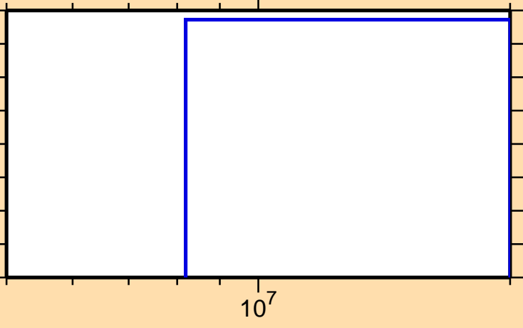
\sigma vs. E for ^{225}\text{At}(n,nt)
