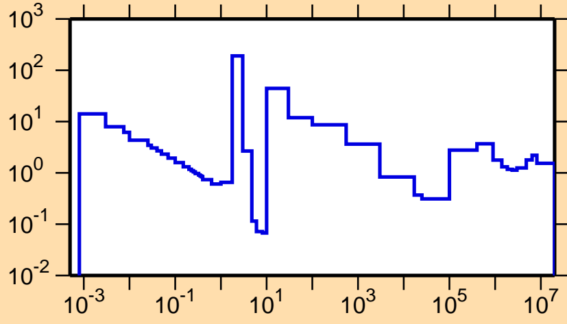
\sigma vs. E for ^{225}\text{At}(n,\text{nonel.})
