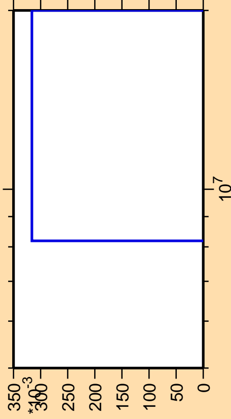
\Delta\sigma/\sigma vs. E for ^{225}\text{At} (mt 42)
