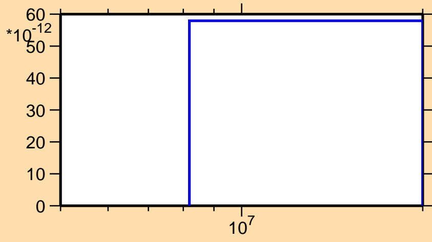
\sigma vs. E for ^{225}\text{At}(\text{mt } 11)
