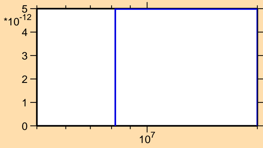
\sigma vs. E for ^{225}\text{At}(n,3n\alpha)
