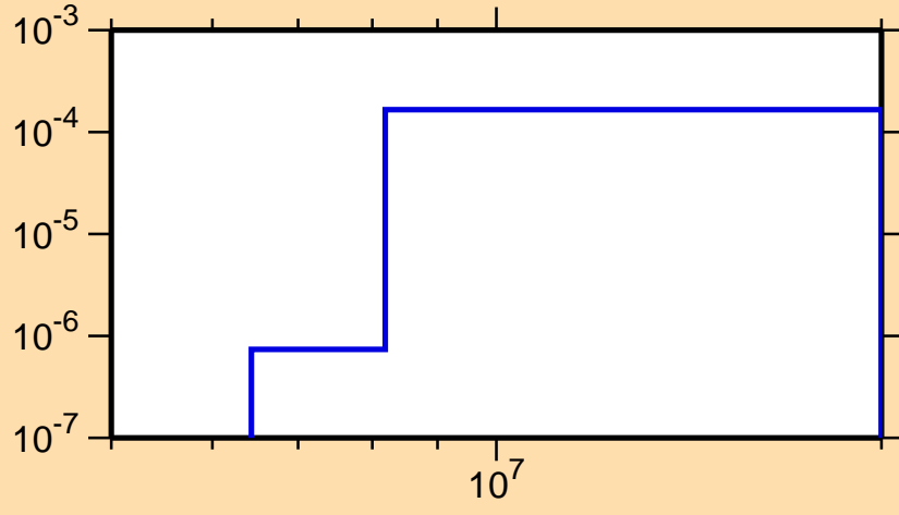
\sigma vs. E for ^{225}\text{At}(n,t)
