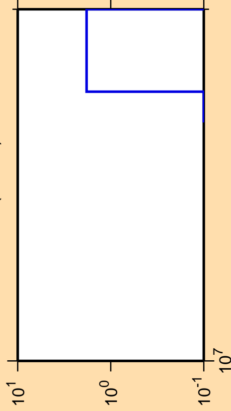
\Delta\sigma/\sigma vs. E for ^{226}\text{At} (mt 42)
