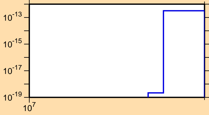
\sigma vs. E for ^{226}\text{At} (mt 42)
