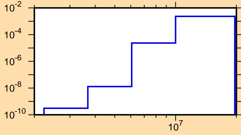
\sigma vs. E for ^{226}\text{At}(n,\alpha)
