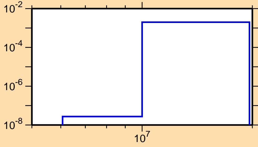
\sigma vs. E for ^{226}\text{At}(n,n\alpha)
