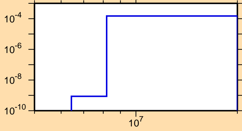
\sigma vs. E for ^{226}\text{At}(n,t)
