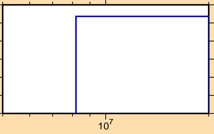
\sigma vs. E for ^{226}\text{At}(n,nt)
