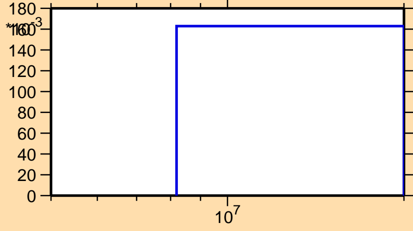
\sigma vs. E for ^{226}\text{At}(n,3n)
