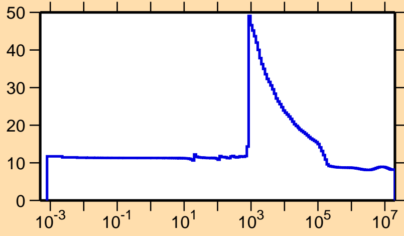
\sigma vs. E for ^{227}\text{At}(n,\text{el.})
