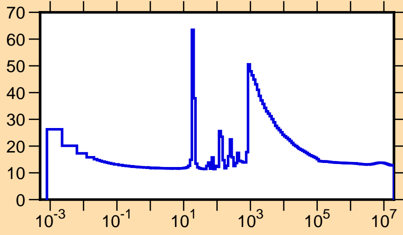
\sigma vs. E for ^{227}\text{At}(n,\text{tot.})
