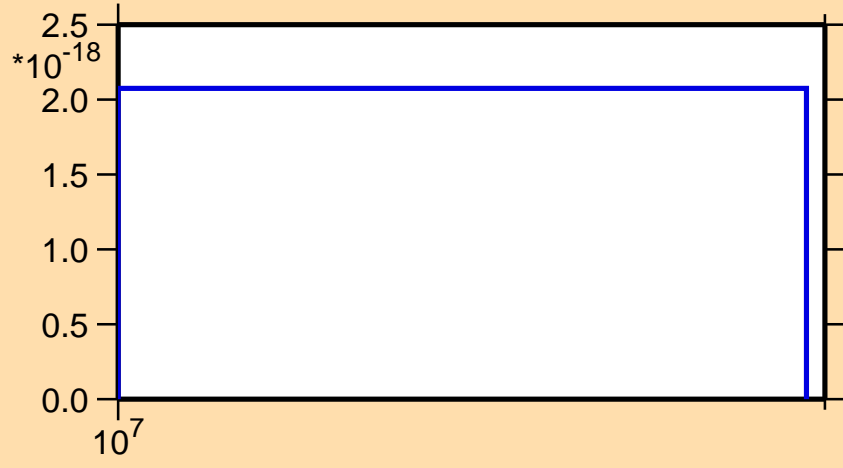
\sigma vs. E for ^{227}\text{At}(\text{mt } 42)
