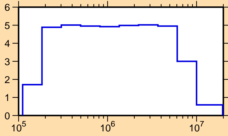
\sigma vs. E for ^{227}\text{At}(n,\text{inel.})
