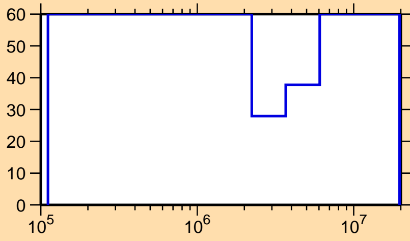
\Delta\sigma/\sigma vs. E for ^{227}\text{At}(n,\text{el.})
