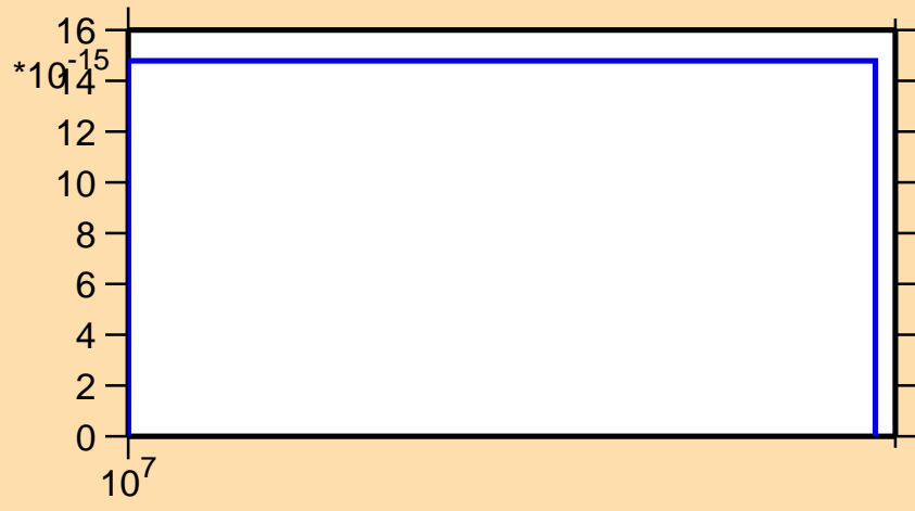
\sigma vs. E for ^{227}\text{At}(\text{mt } 11)
