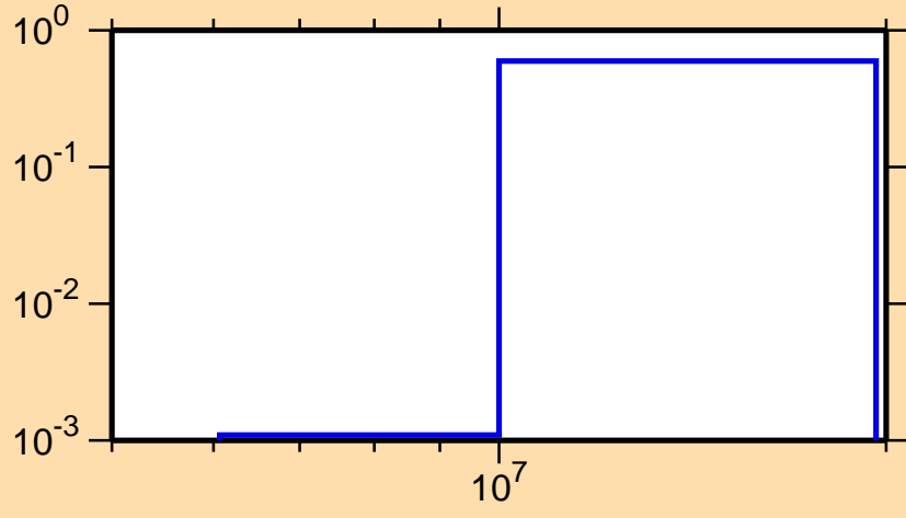
\sigma vs. E for ^{227}\text{At}(n,3n)
