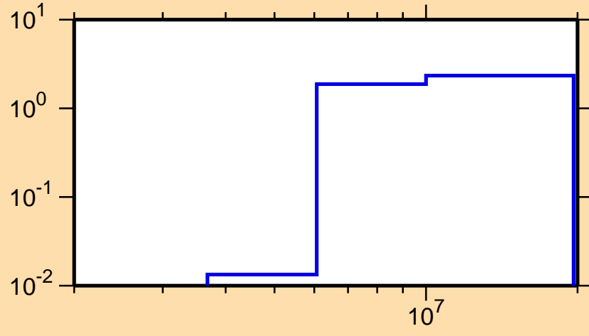
\sigma vs. E for ^{227}\text{At}(n,2n)
