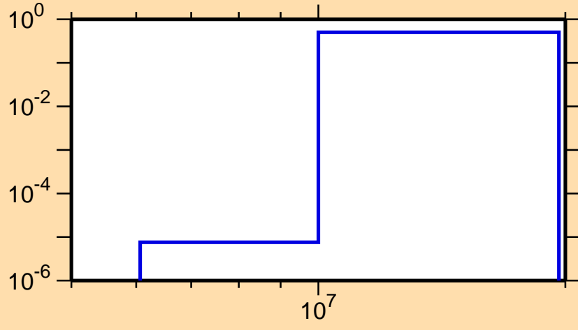
\sigma vs. E for ^{227}\text{At}(n,t)
