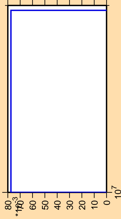
\Delta\sigma/\sigma vs. E for ^{227}\text{At}(\text{mt } 11)
