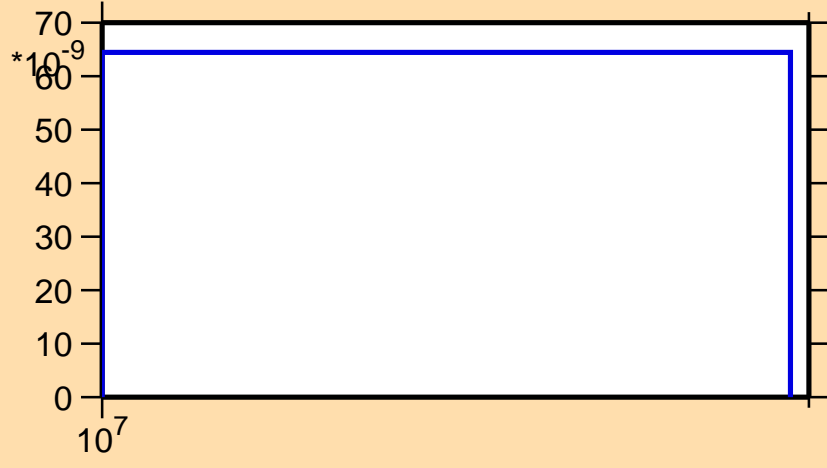
\sigma vs. E for ^{227}\text{At}(n,2np)
