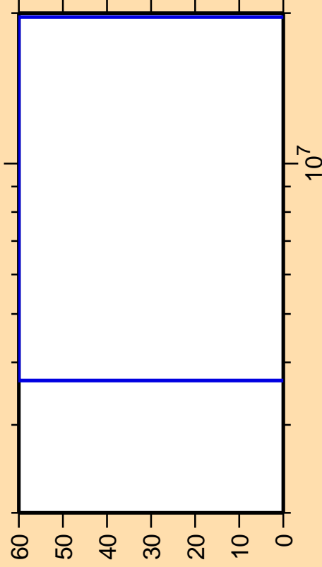
\Delta\sigma/\sigma vs. E for ^{227}\text{At}(n,n\text{cont.})
