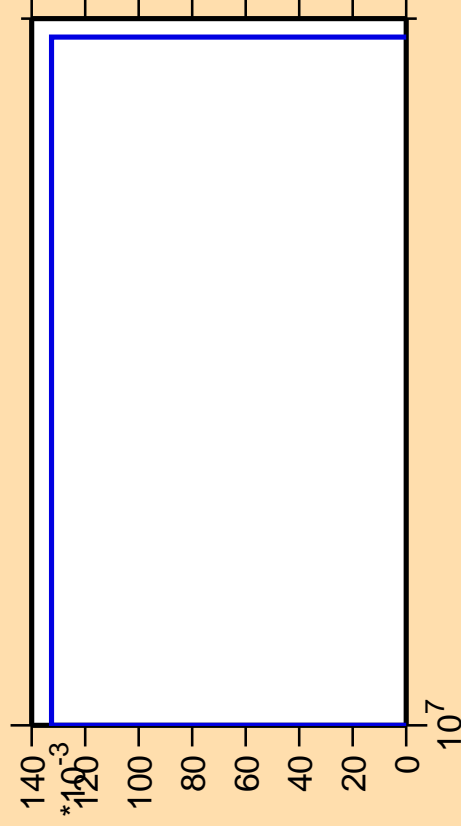
\Delta\sigma/\sigma vs. E for ^{227}\text{At}(n,3n\alpha)
