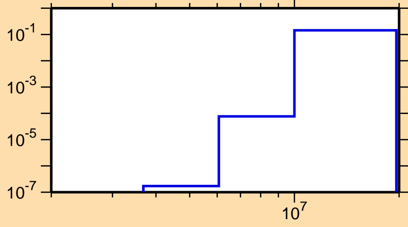
\sigma vs. E for ^{227}\text{At}(n,\alpha)
