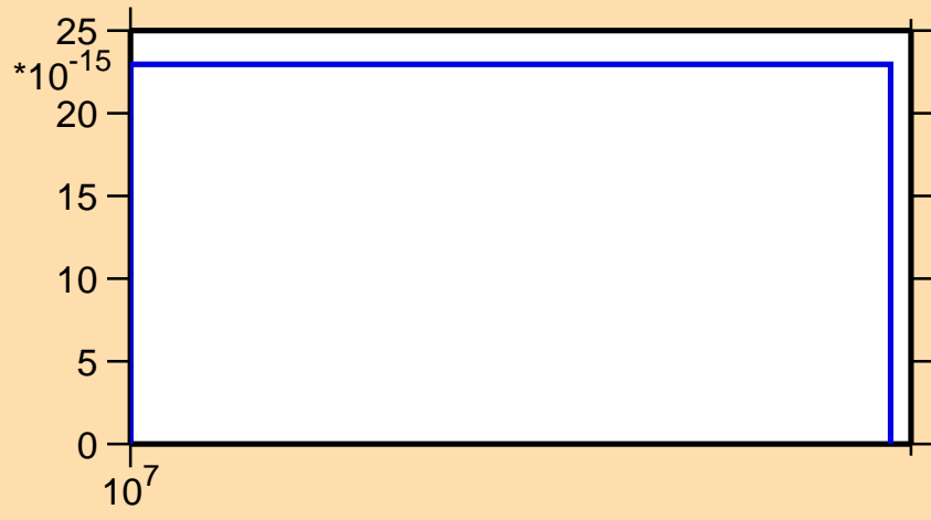
\sigma vs. E for ^{227}\text{At}(n,3n\alpha)
