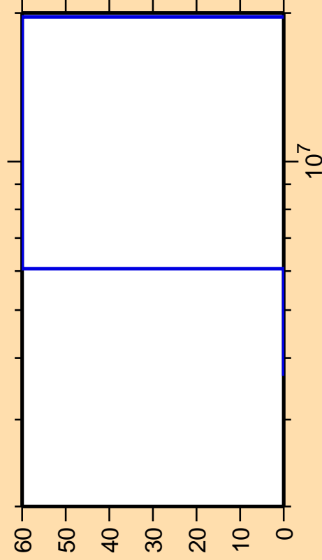
\Delta\sigma/\sigma vs. E for ^{227}\text{At}(n,f)
