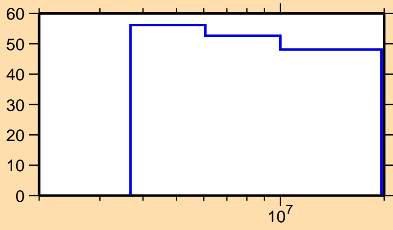
\Delta\sigma/\sigma vs. E for ^{227}\text{At}(n,\text{nonel.})
