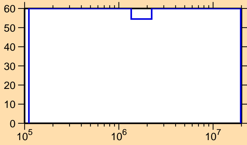
\Delta\sigma/\sigma vs. E for ^{227}\text{At}(n,n\text{cont.})
