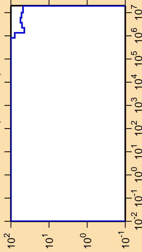
\Delta\sigma/\sigma vs. E for ^{227}\text{At}(n,\text{nonel.})
