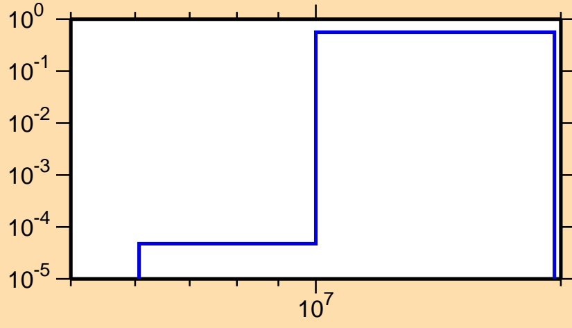
\sigma vs. E for ^{227}\text{At}(n,n\alpha)
