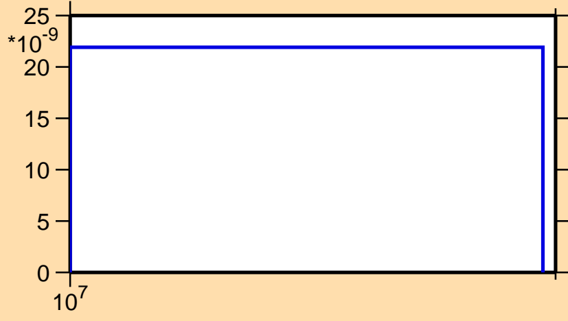
\sigma vs. E for ^{227}\text{At}(n,2n\alpha)
