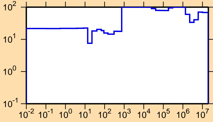
\Delta\sigma/\sigma vs. E for ^{227}\text{At}(n,\text{tot.})
