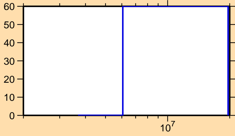
\Delta\sigma/\sigma vs. E for ^{227}\text{At}(n,f)
