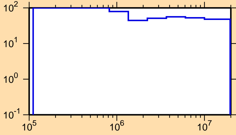
\Delta\sigma/\sigma vs. E for ^{227}\text{At}(n,\text{nonel.})
