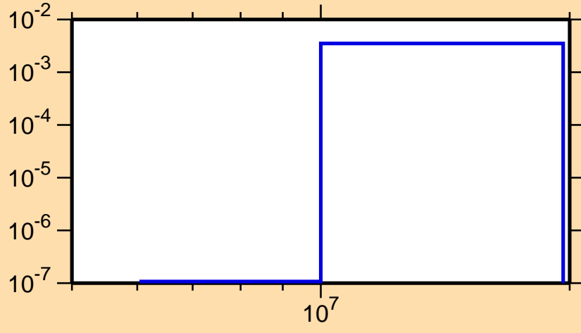
\sigma vs. E for ^{227}\text{At}(n,p)
