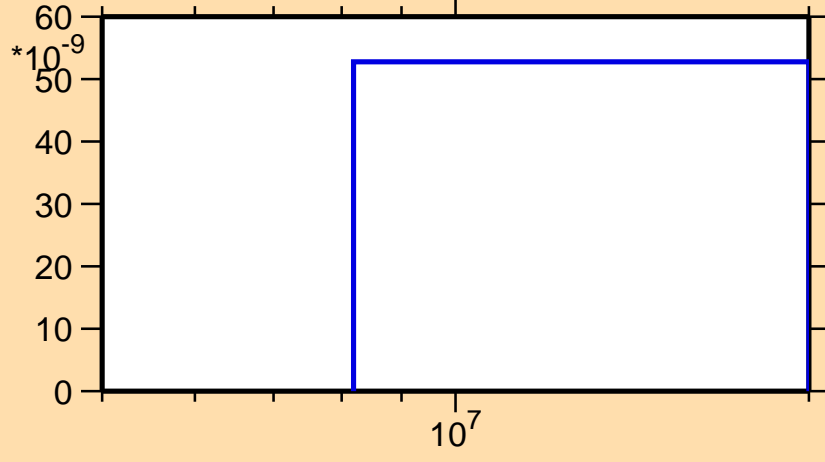
\sigma vs. E for ^{227}\text{At}(n,nt)
