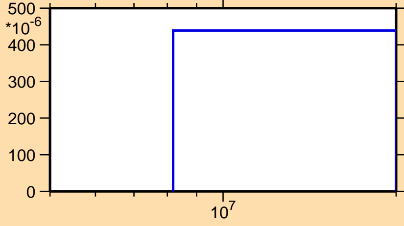
\sigma vs. E for ^{227}\text{At}(n,np)
