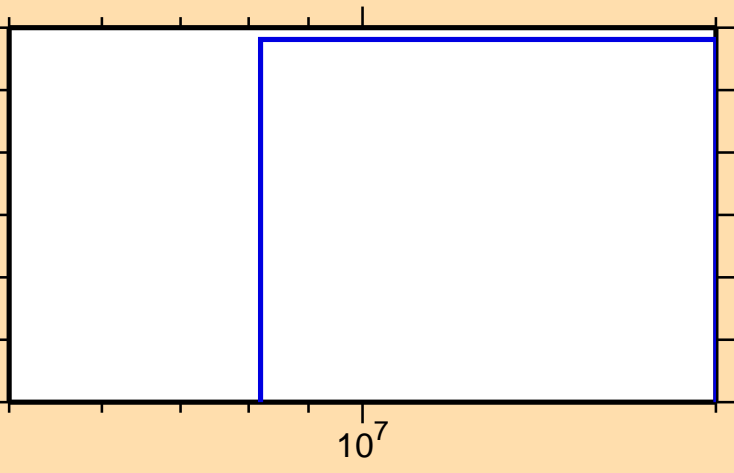
\sigma vs. E for ^{227}\text{At}(n,2np)
