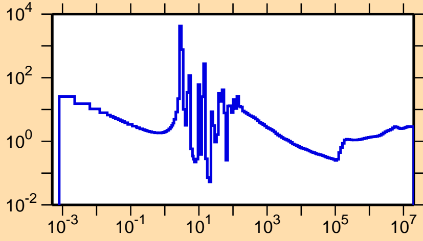
\sigma vs. E for ^{228}\text{At}(n,\text{nonel.})
