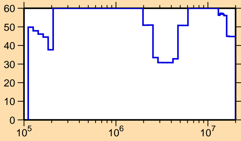
\Delta\sigma/\sigma vs. E for ^{228}\text{At}(n, el.)
