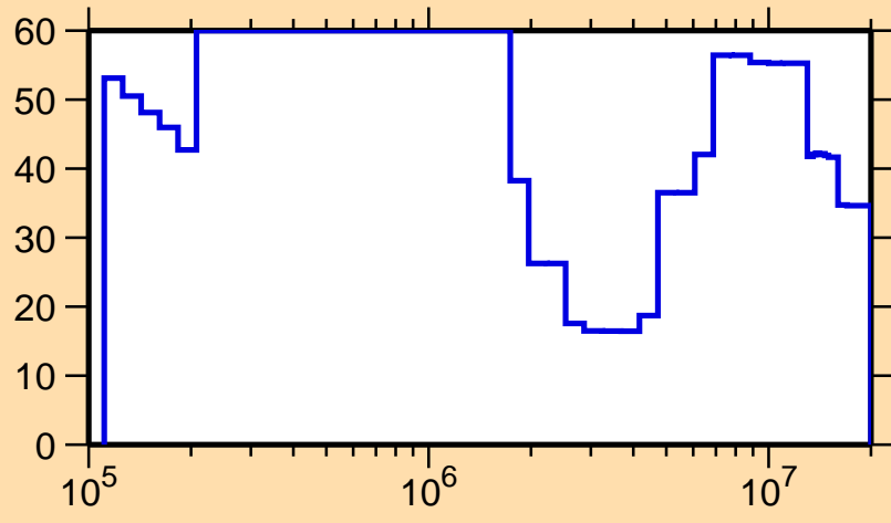
\Delta\sigma/\sigma vs. E for ^{228}\text{At}(n,\text{tot.})
