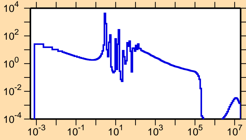
\sigma vs. E for ^{228}\text{At}(n,\gamma)
