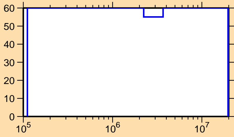
\Delta\sigma/\sigma vs. E for ^{228}\text{At}(n,\text{inel.})
