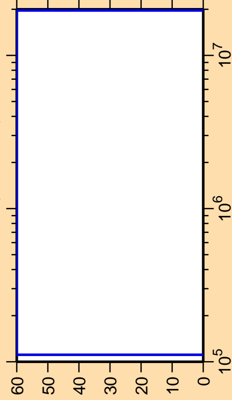
\Delta\sigma/\sigma vs. E for ^{228}\text{At}(n,n\text{cont.})
