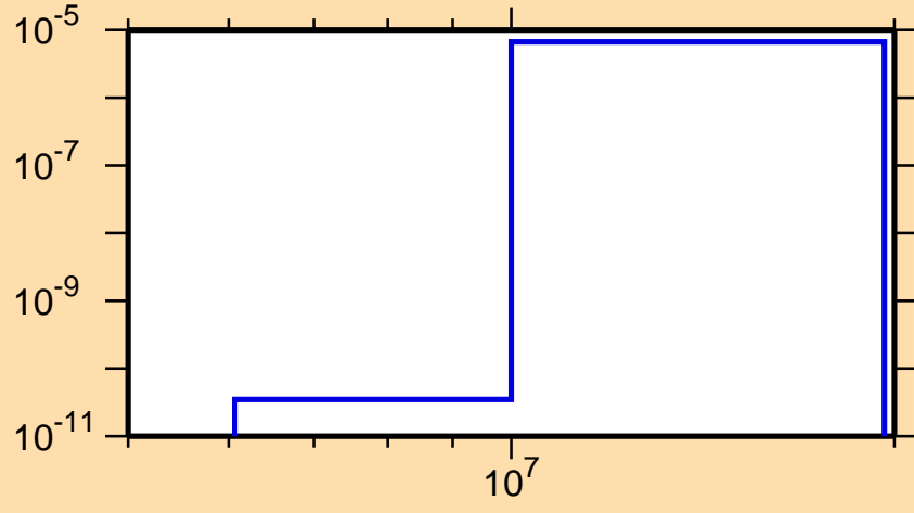
\sigma vs. E for ^{228}\text{At}(n,n\alpha)
