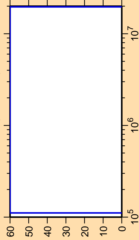
\Delta\sigma/\sigma vs. E for ^{228}\text{At}(n,\text{ncont.})
