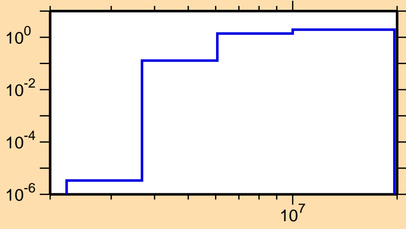
\sigma vs. E for ^{228}\text{At}(n,2n)
