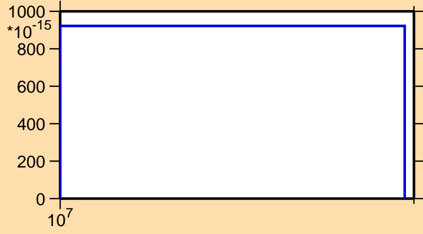
\sigma vs. E for ^{228}\text{At} (mt 11)
