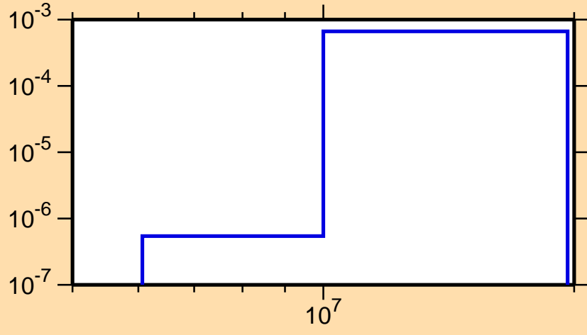
\sigma vs. E for ^{228}\text{At}(n,t)
