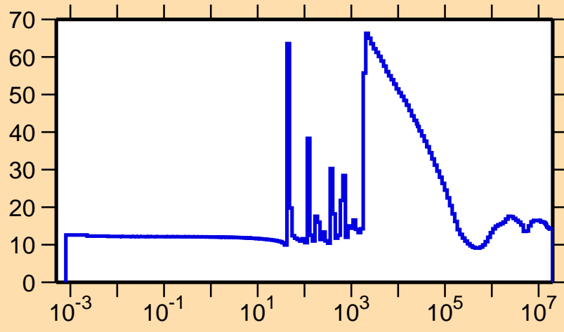
\sigma vs. E for ^{229}\text{At}(n,\text{el.})
