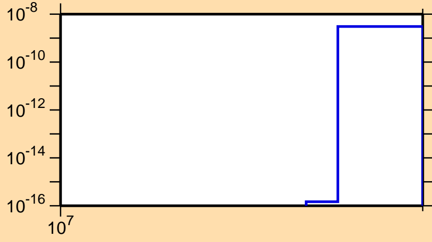
\sigma vs. E for ^{229}\text{At}(\text{mt } 11)
