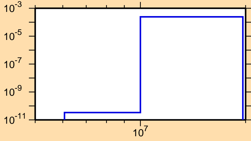
\sigma vs. E for ^{229}\text{At}(n,p)
