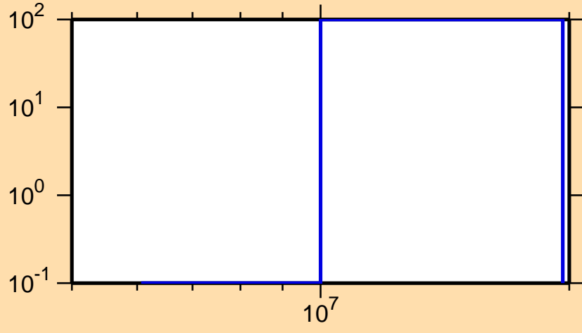
\Delta\sigma/\sigma vs. E for ^{229}\text{At}(n,f)
