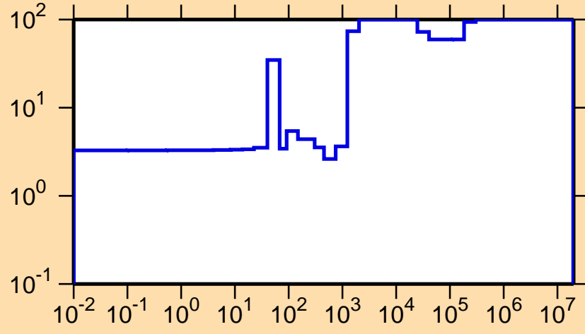
\Delta\sigma/\sigma vs. E for ^{229}\text{At}(n,el.)
