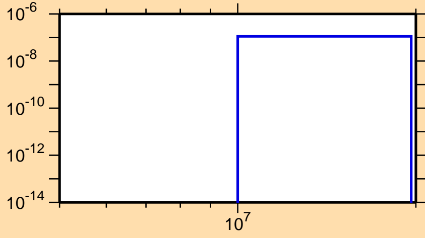
\sigma vs. E for ^{229}\text{At}(n,n\alpha)
