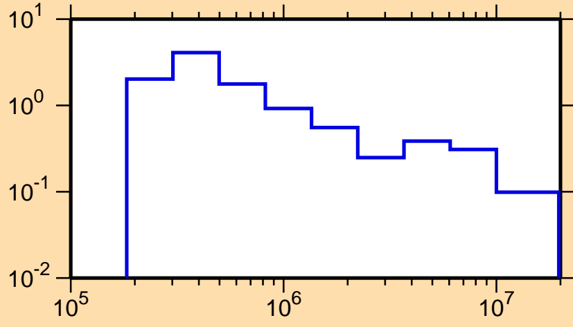
\sigma vs. E for ^{229}\text{At}(n,n_1)
