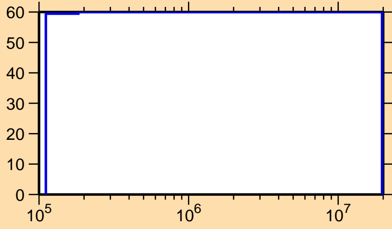
\Delta\sigma/\sigma vs. E for ^{229}\text{At}(n,\text{el.})
