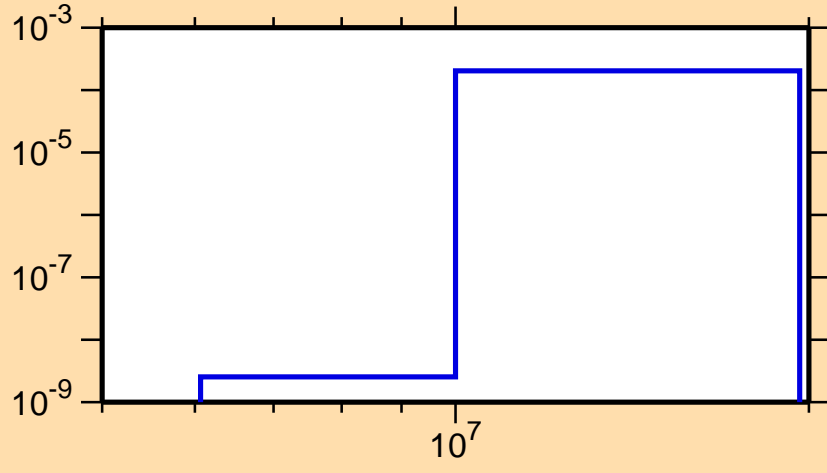
\sigma vs. E for ^{229}\text{At}(n,\alpha)
