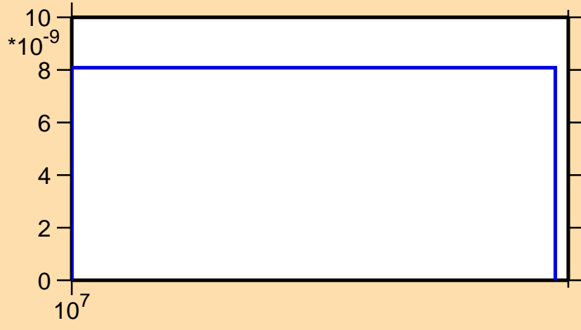
\sigma vs. E for ^{229}\text{At}(n,\text{nd})
