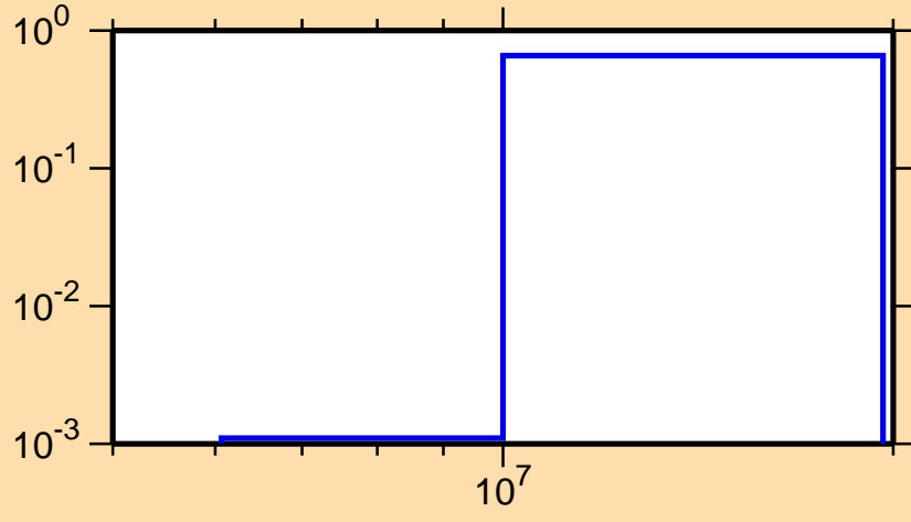
\sigma vs. E for ^{229}\text{At}(n,3n)
