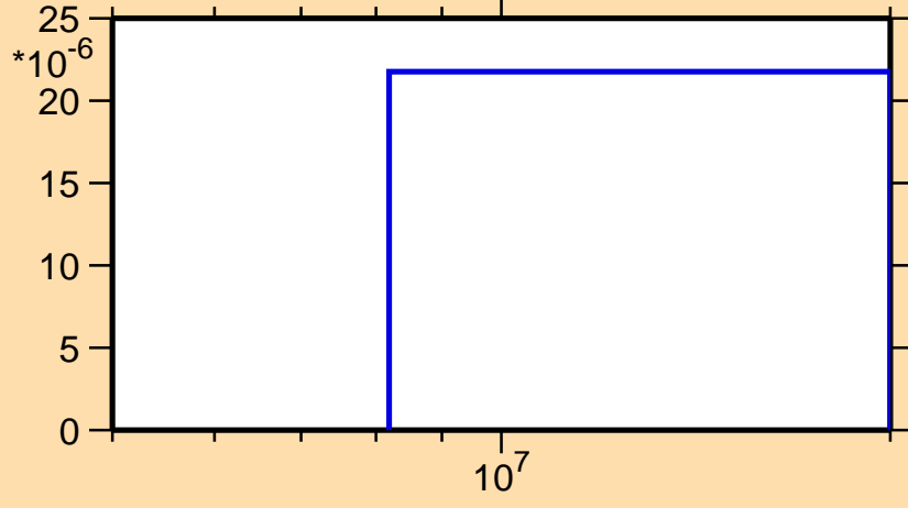
\sigma vs. E for ^{229}\text{At}(n,t)
