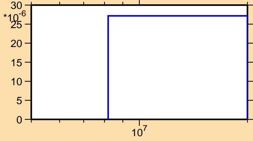
\sigma vs. E for ^{229}\text{At}(n,d)
