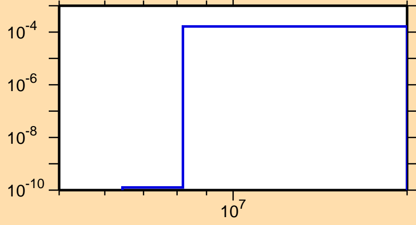
\sigma vs. E for ^{229}\text{At}(n,\alpha)
