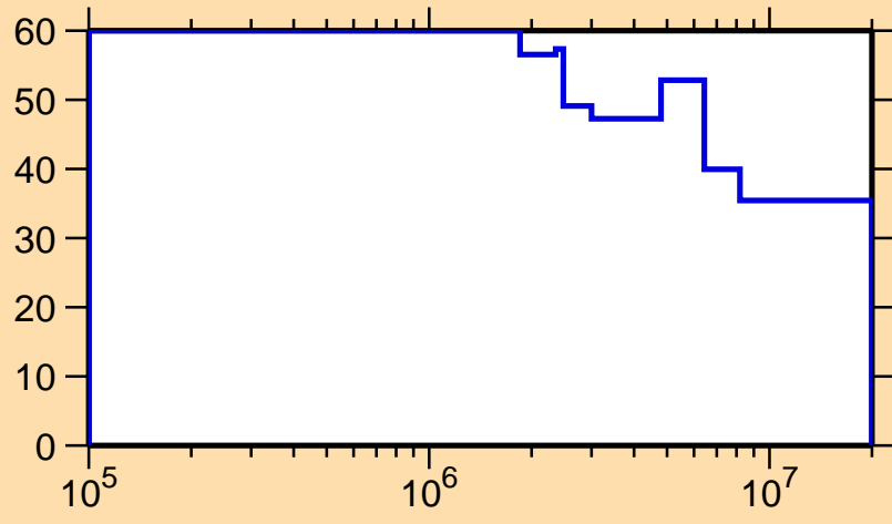
\Delta\sigma/\sigma vs. E for ^{229}\text{At}(n,\text{nonel.})
