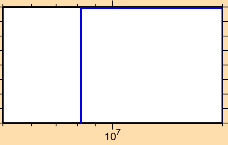
\sigma vs. E for ^{229}\text{At}(n,\text{nd})
