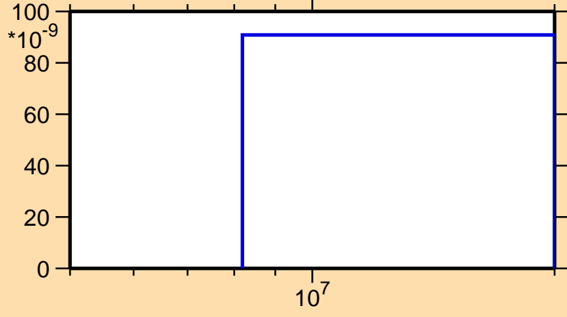
\sigma vs. E for ^{229}\text{At}(n,n\alpha)
