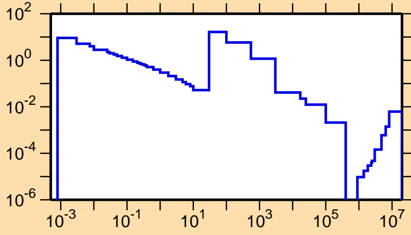
\sigma vs. E for ^{229}\text{At}(n,\gamma)
