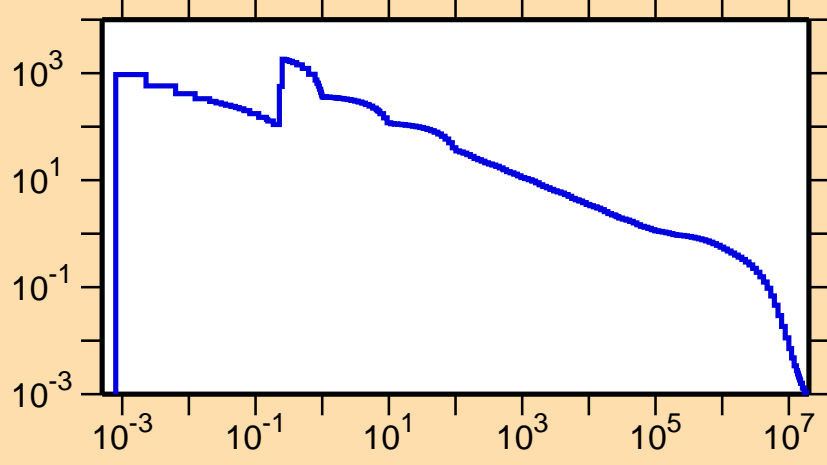
\sigma vs. E for ^{176}\text{Au}(n,\gamma)
