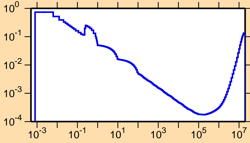
\sigma vs. E for ^{176}\text{Au}(n,p\alpha)
