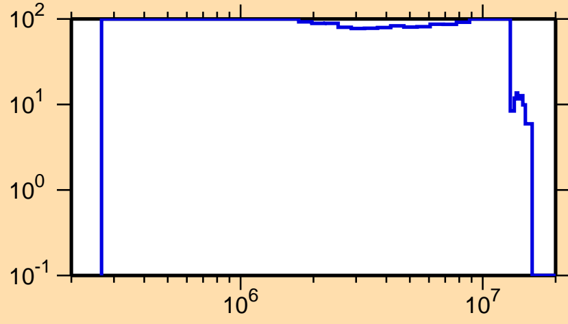
\Delta\sigma/\sigma vs. E for ^{176}\text{Au}(n,n_1)
