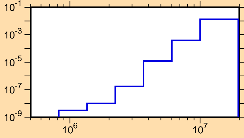
\sigma vs. E for ^{176}\text{Au}(n,n\alpha)
