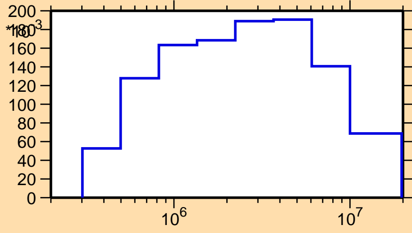
\sigma vs. E for ^{176}\text{Au}(n,n_4)
