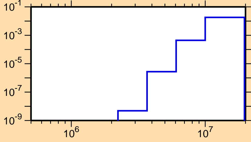
\sigma vs. E for ^{176}\text{Au}(n,d)
