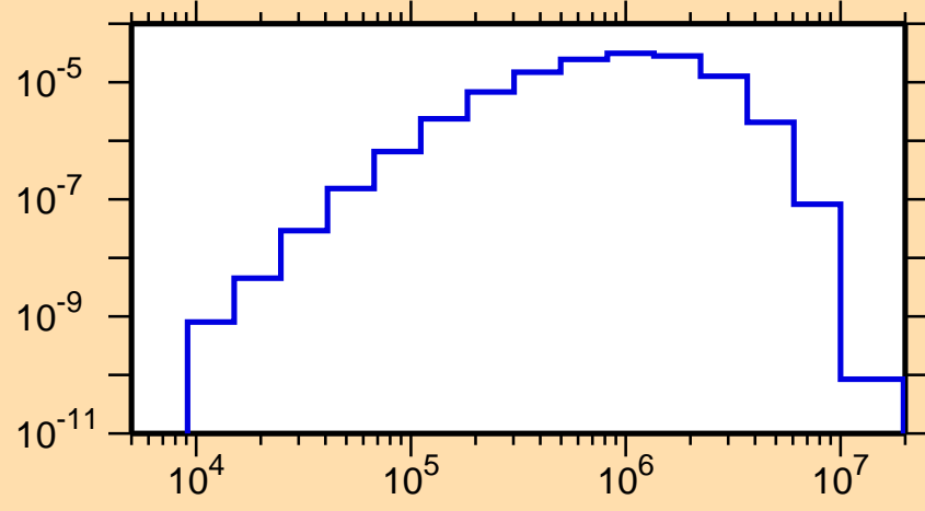
\sigma vs. E for ^{176}\text{Au}(n,n_2)
