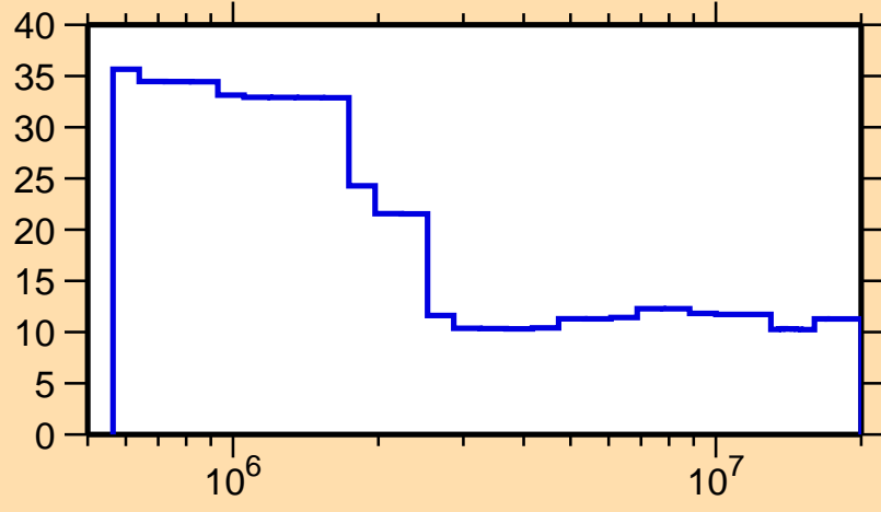
\Delta\sigma/\sigma vs. E for ^{177}\text{Au}(n,n\text{onel.})
