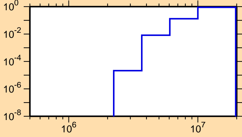
\sigma vs. E for ^{177}\text{Au}(n,np)
