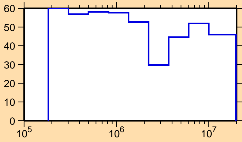
\Delta\sigma/\sigma vs. E for ^{177}\text{Au}(n,n_1)
