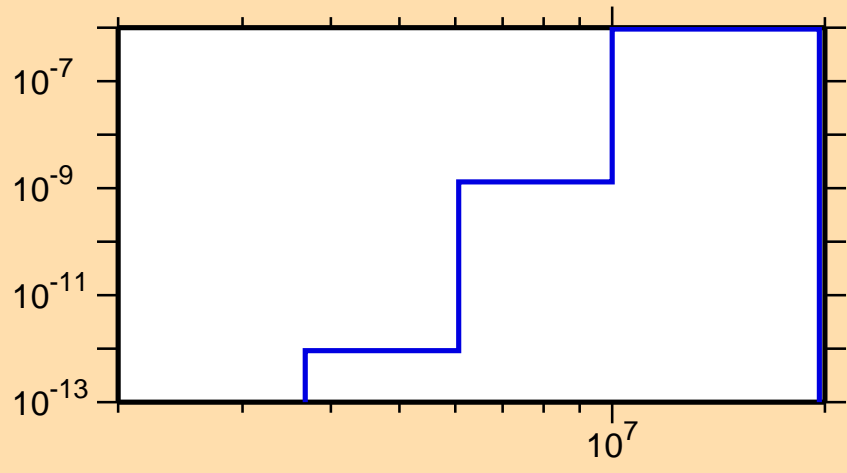
\sigma vs. E for ^{177}\text{Au}(\text{mt117})
