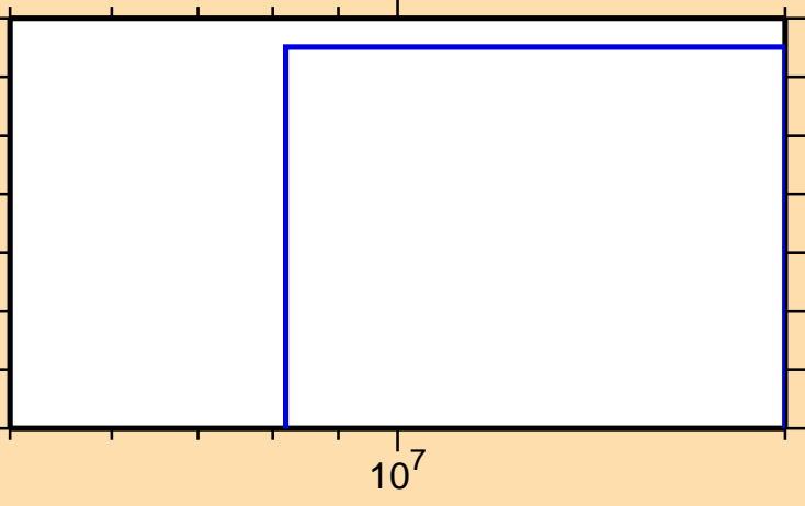
\sigma vs. E for ^{177}\text{Au}(n,2n\alpha)
