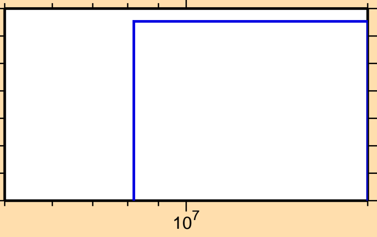
\sigma vs. E for ^{177}\text{Au}(n,\text{pt})
