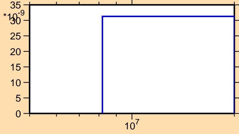
\sigma vs. E for ^{177}\text{Au}(n,\text{nd})
