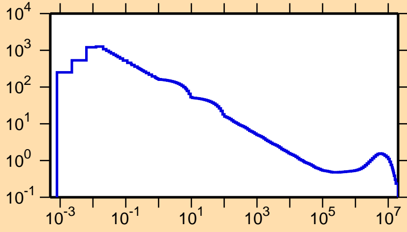
\sigma vs. E for ^{177}\text{Au}(n,p)
