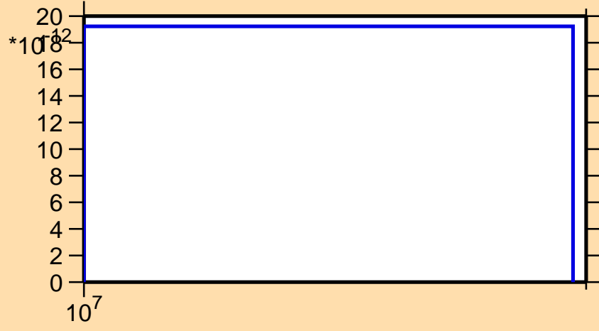
\sigma vs. E for ^{177}\text{Au} (mt 34)
