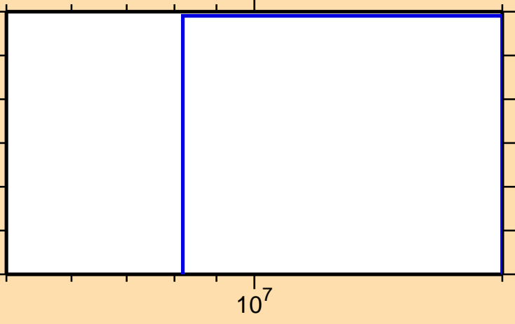
\sigma vs. E for ^{177}\text{Au}(n,2n)
