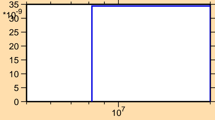
\sigma vs. E for ^{177}\text{Au}(n,nd)
