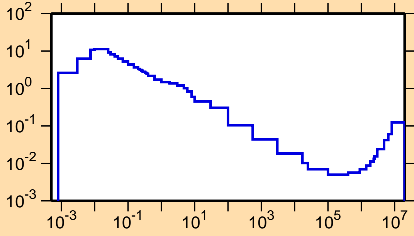
\sigma vs. E for ^{177}\text{Au}(n,\alpha)
