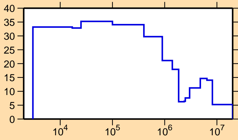
\Delta\sigma/\sigma vs. E for ^{177}\text{Au}(n, tot.)
