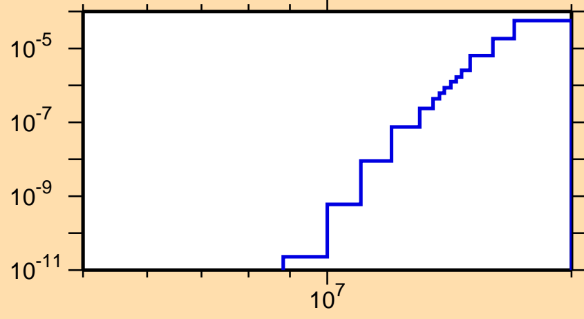
\sigma vs. E for ^{178}\text{Au}(n,\text{pd})
