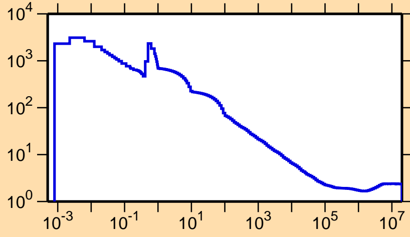
\sigma vs. E for ^{178}\text{Au}(n,\text{nonel.})
