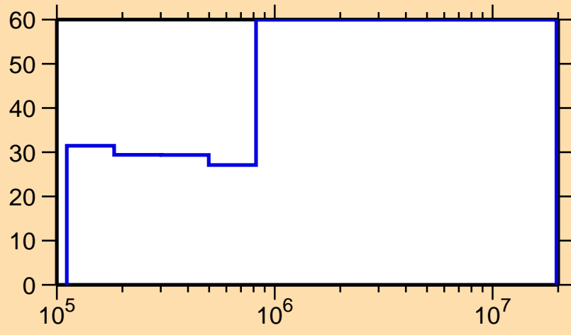
\Delta\sigma/\sigma vs. E for ^{178}\text{Au}(n,n_1)
