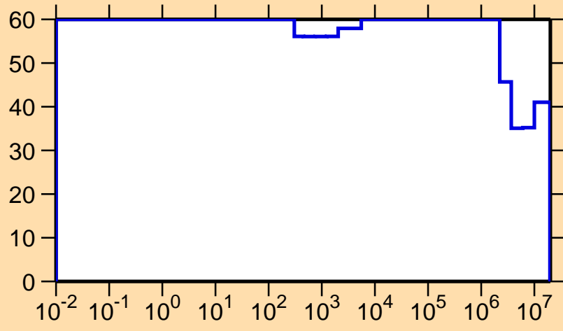
\Delta\sigma/\sigma vs. E for ^{178}\text{Au}(n,p)
