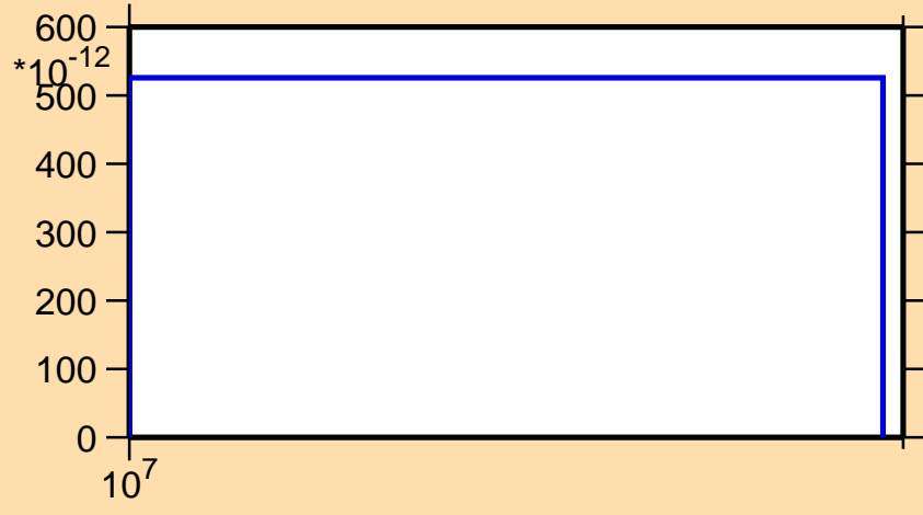
\sigma vs. E for ^{178}\text{Au}(\text{mt } 34)
