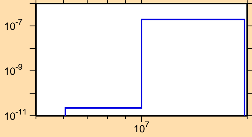
\sigma vs. E for ^{178}\text{Au}(\text{mt117})
