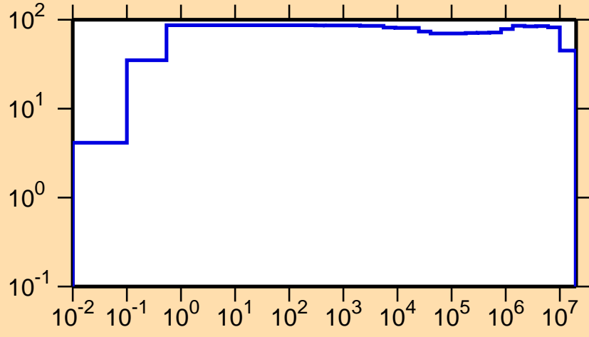
\Delta\sigma/\sigma vs. E for ^{178}\text{Au}(n,\gamma)
