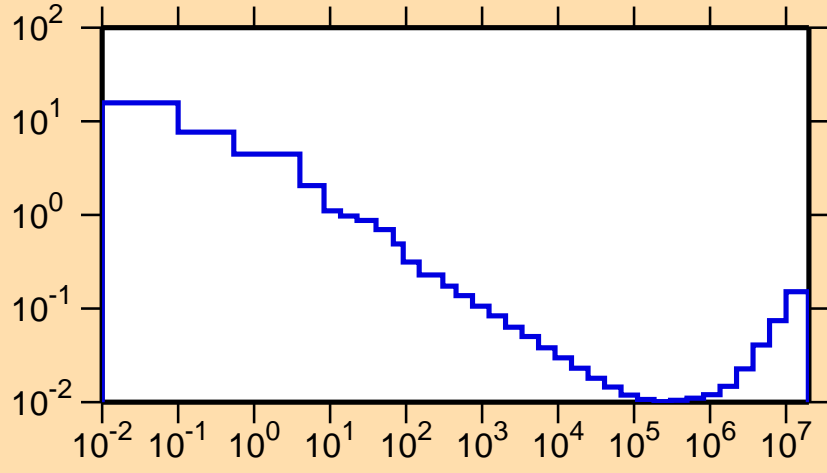
\sigma vs. E for ^{178}\text{Au}(n,\alpha)
