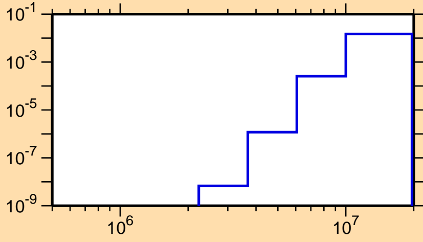
\sigma vs. E for ^{178}\text{Au}(n,d)
