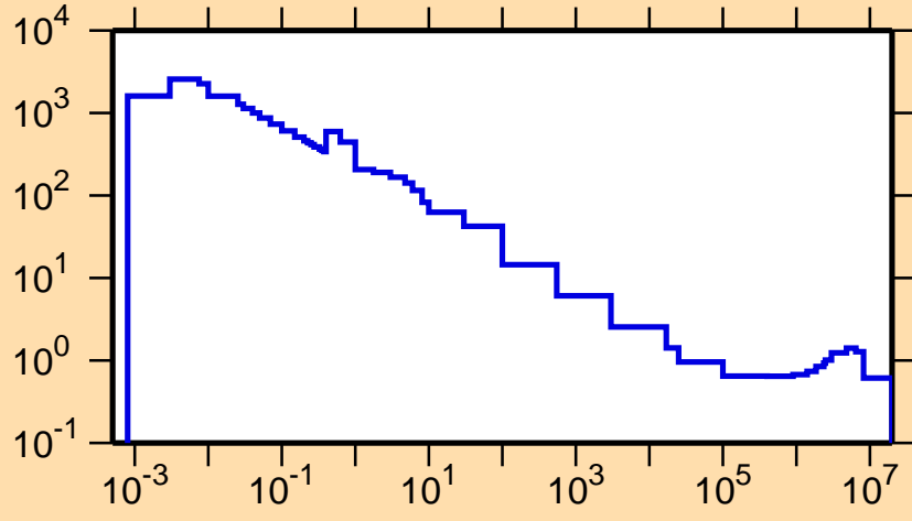
\sigma vs. E for ^{178}\text{Au}(n,p)
