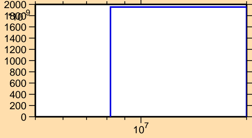
\sigma vs. E for ^{178}\text{Au}(n,nd)
