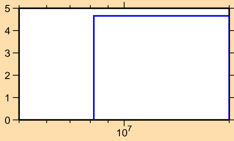
\Delta\sigma/\sigma vs. E for ^{178}\text{Au}(n,\text{tot.})
