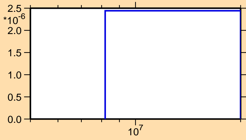
\sigma vs. E for ^{178}\text{Au}(n,\text{pd})
