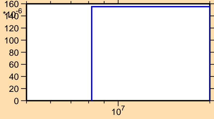
\sigma vs. E for ^{178}\text{Au}(n,2n\alpha)
