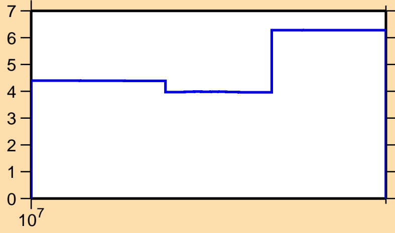
\Delta\sigma/\sigma vs. E for ^{179}\text{Au}(n,\text{tot.})
