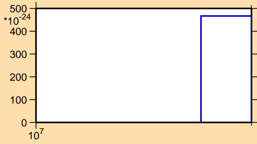
\sigma vs. E for ^{179}\text{Au}(\text{mt } 42)
