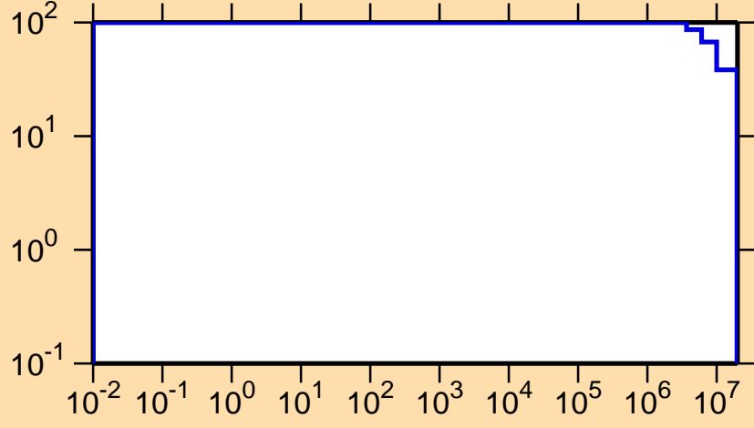
\Delta\sigma/\sigma vs. E for ^{179}\text{Au}(n,p)
