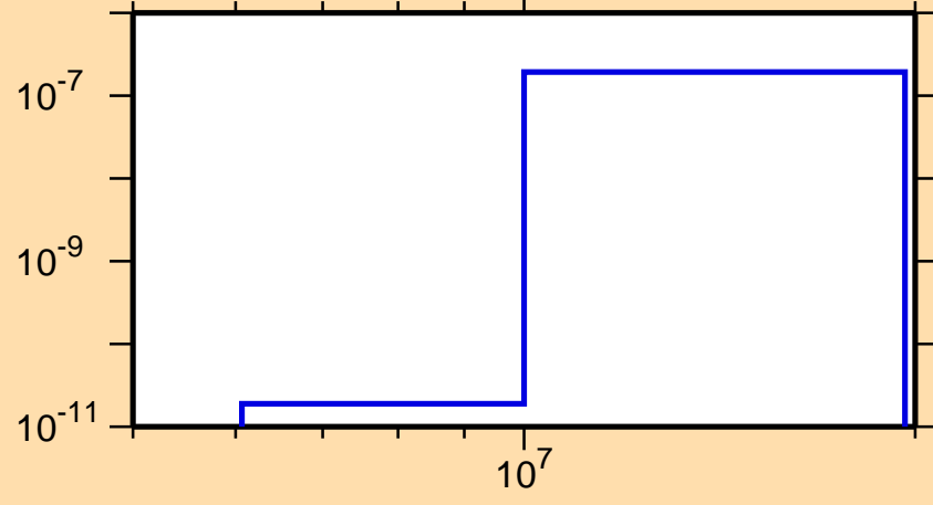
\sigma vs. E for ^{179}\text{Au}(\text{mt117})
