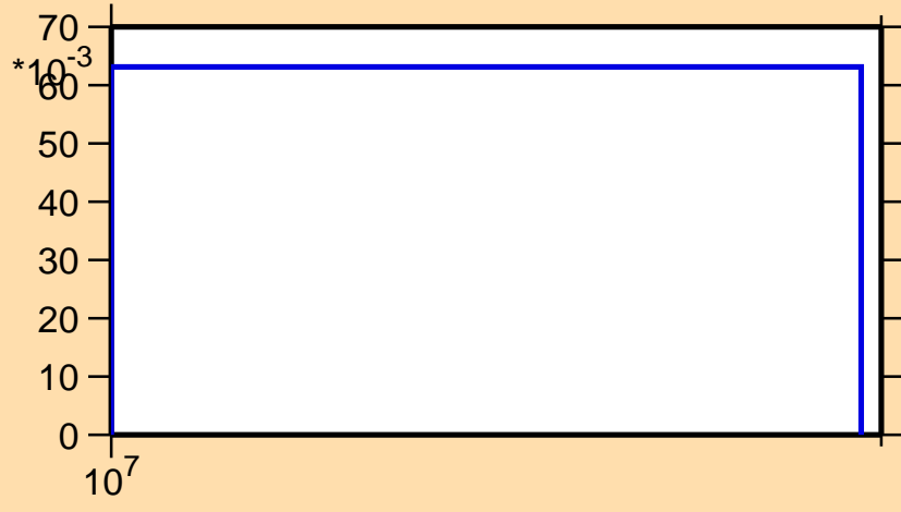
\sigma vs. E for ^{179}\text{Au}(n,2n)
