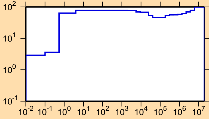
\Delta\sigma/\sigma vs. E for ^{179}\text{Au}(n,\gamma)
