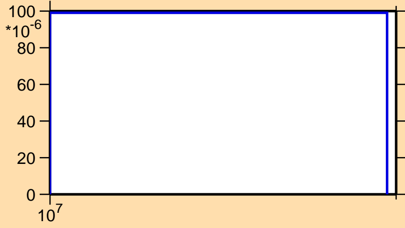
\sigma vs. E for ^{179}\text{Au}(n,2np)
