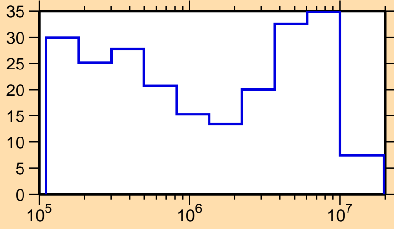
\Delta\sigma/\sigma vs. E for ^{179}\text{Au}(n,\text{el.})
