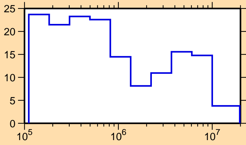
\Delta\sigma/\sigma vs. E for ^{179}\text{Au}(n,\text{tot.})
