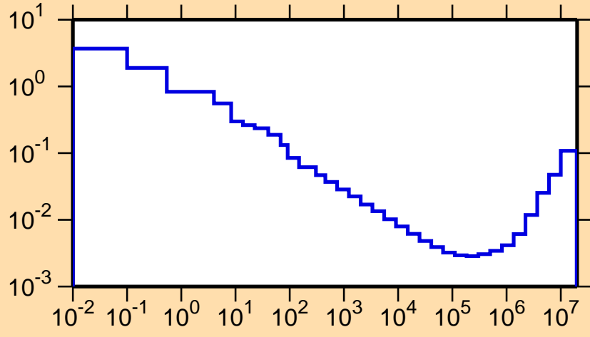
\sigma vs. E for ^{179}\text{Au}(n,\alpha)
