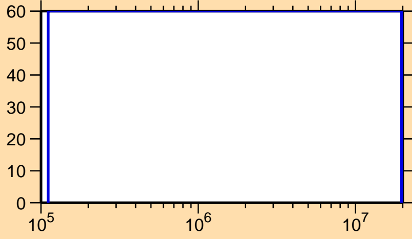
\Delta\sigma/\sigma vs. E for ^{179}\text{Au}(n,n_1)
