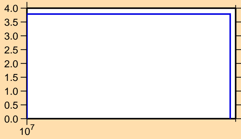
\Delta\sigma/\sigma vs. E for ^{179}\text{Au}(n,\text{tot.})
