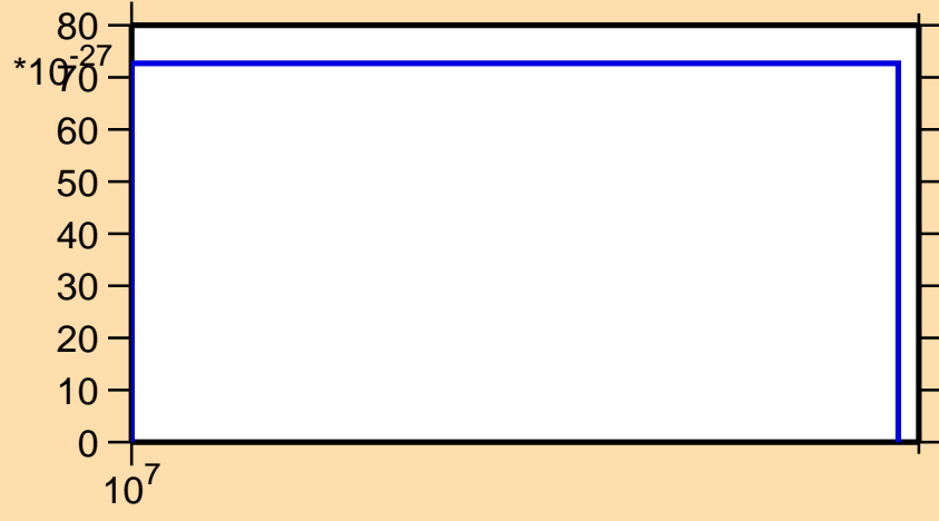
\sigma vs. E for ^{179}\text{Au} (mt 42)
