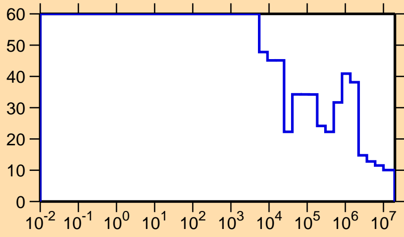
\Delta\sigma/\sigma vs. E for ^{179}\text{Au}(n,\text{nonel.})
