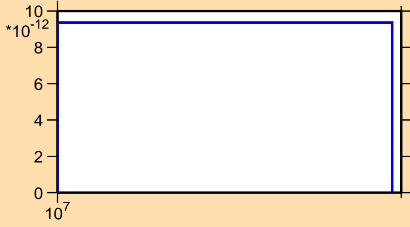
\sigma vs. E for ^{179}\text{Au} (mt 34)
