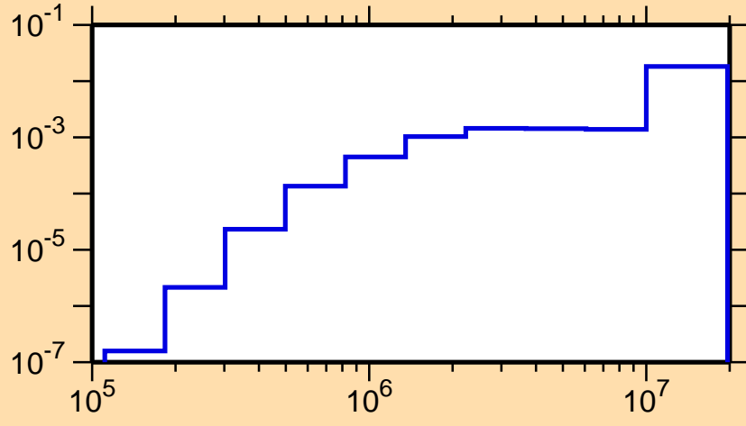
\sigma vs. E for ^{179}\text{Au}(n,n\alpha)
