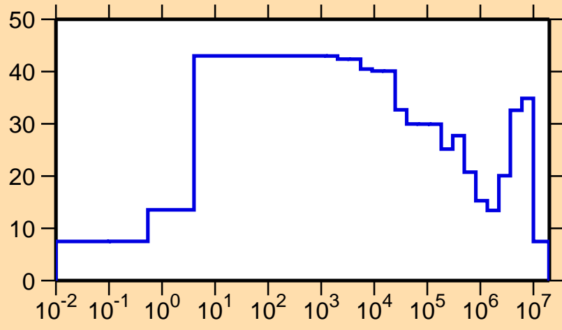
\Delta\sigma/\sigma vs. E for ^{179}\text{Au}(n,\text{el.})
