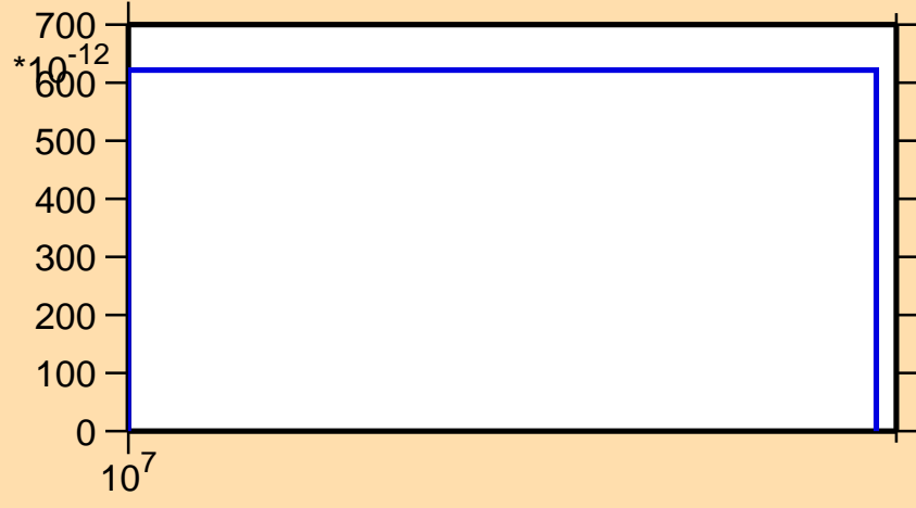
\sigma vs. E for ^{179}\text{Au}(n,pt)
