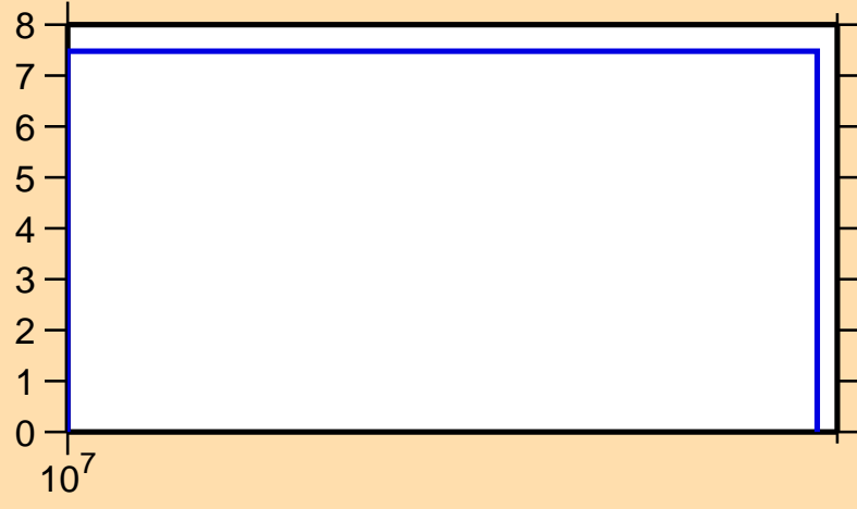
\Delta\sigma/\sigma vs. E for ^{179}\text{Au}(n,\text{el.})
