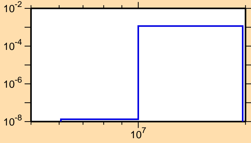
\sigma vs. E for ^{179}\text{Au}(n,2n\alpha)
