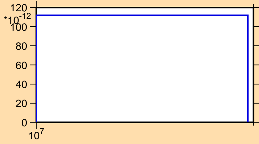
\sigma vs. E for ^{179}\text{Au}(n,nt)
