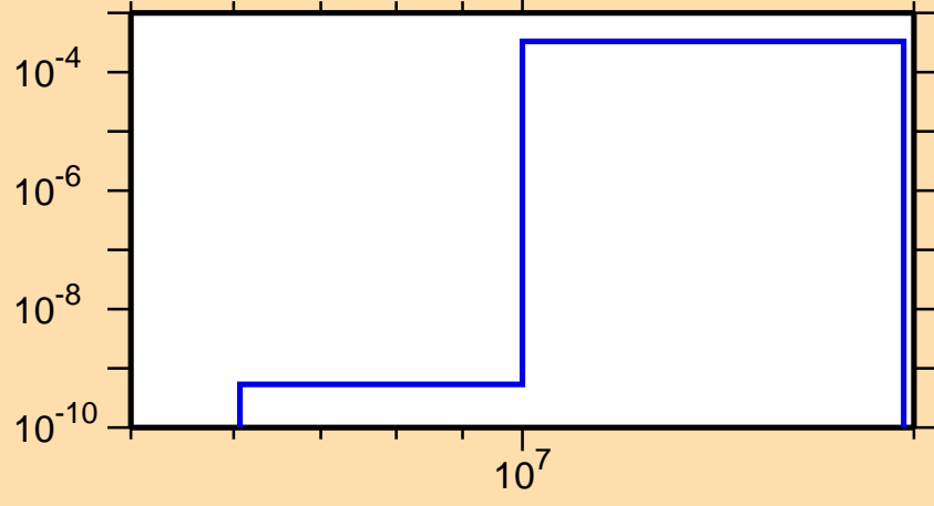
\sigma vs. E for ^{179}\text{Au}(n,t)
