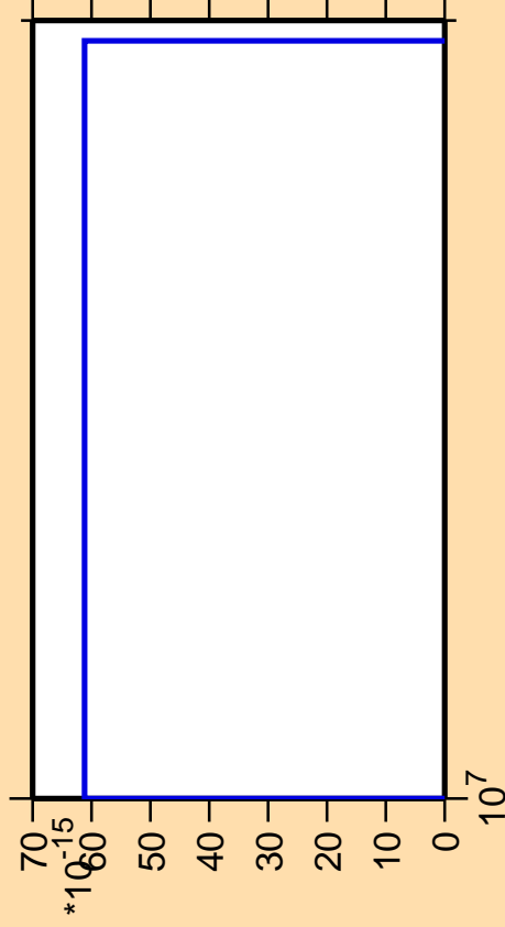
\Delta\sigma/\sigma vs. E for ^{179}\text{Au} (mt 42)
