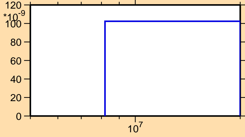
\sigma vs. E for ^{179}\text{Au}(n,nd)
