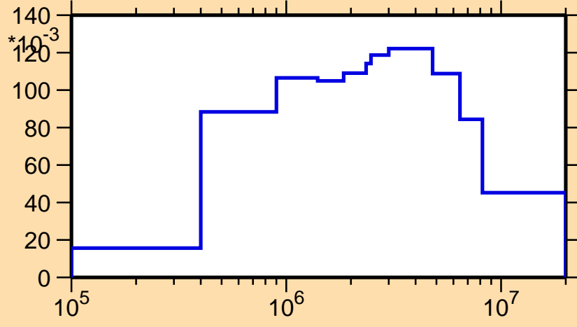
\sigma vs. E for ^{179}\text{Au}(n,n_1)
