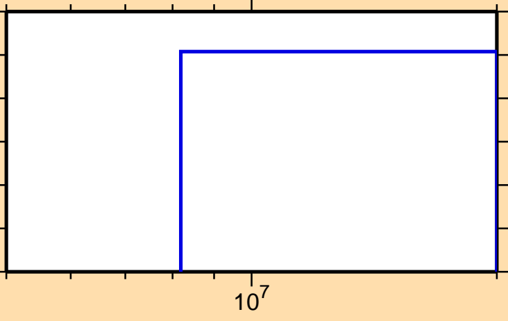
\sigma vs. E for ^{179}\text{Au}(n,2n)
