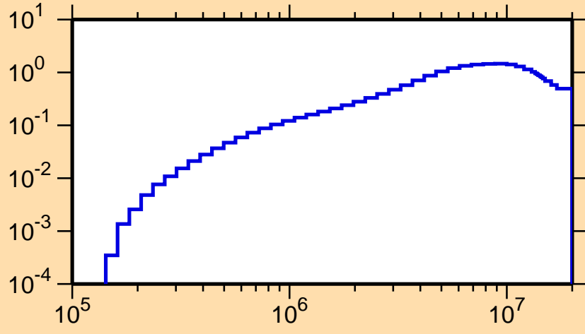
\sigma vs. E for ^{180}\text{Au}(n,n\text{cont.})
