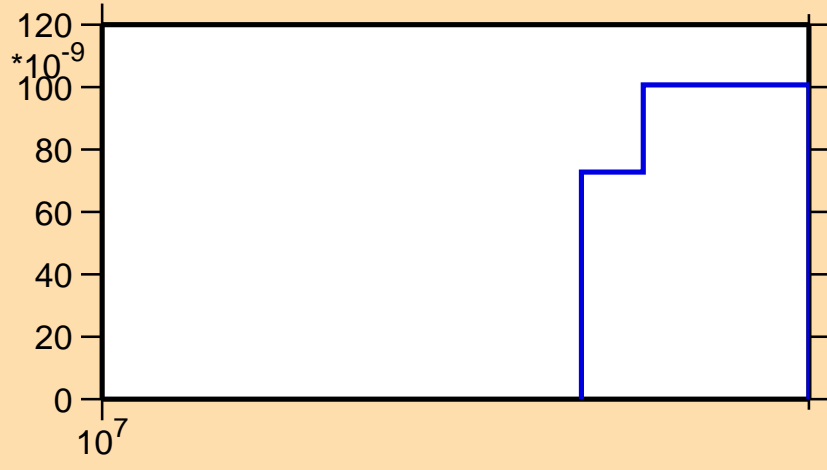
\sigma vs. E for ^{180}\text{Au}(n,3n\alpha)
