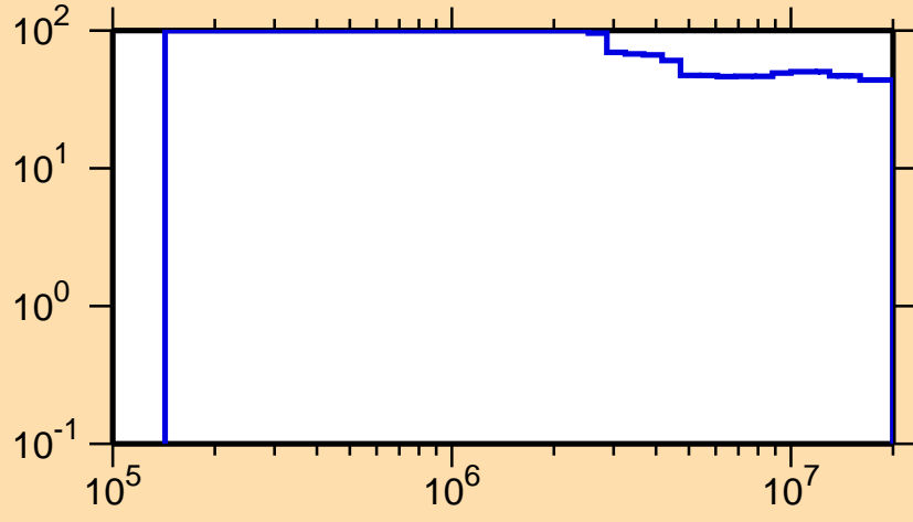
\Delta\sigma/\sigma vs. E for ^{180}\text{Au}(n,n\text{cont.})
