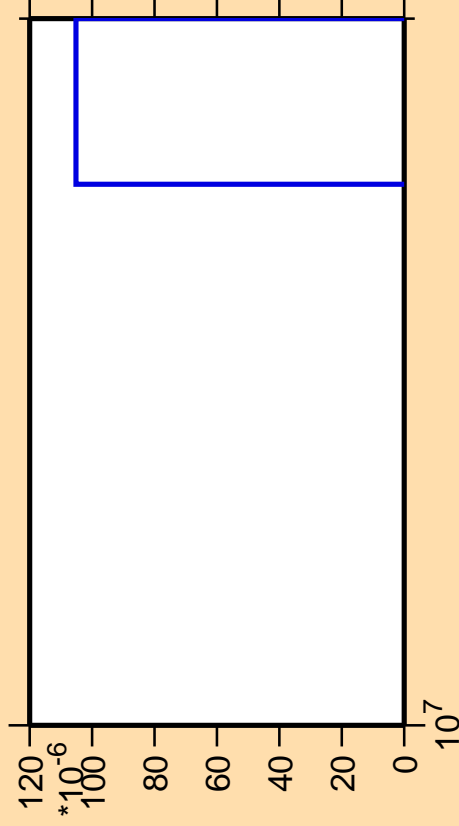
\Delta\sigma/\sigma vs. E for ^{180}\text{Au}(\text{mt } 42)
