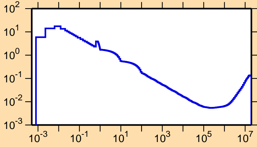
\sigma vs. E for ^{180}\text{Au}(n,\alpha)
