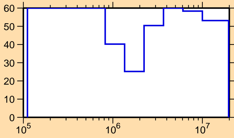
\Delta\sigma/\sigma vs. E for ^{180}\text{Au}(n,n_1)
