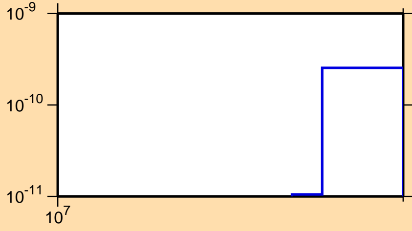
\sigma vs. E for ^{181}\text{Au}(\text{mt } 34)
