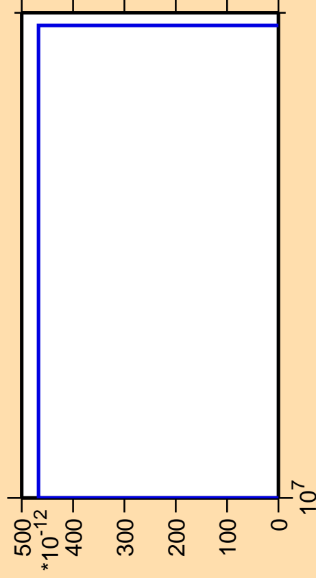
\Delta\sigma/\sigma vs. E for ^{181}\text{Au} (mt 42)
