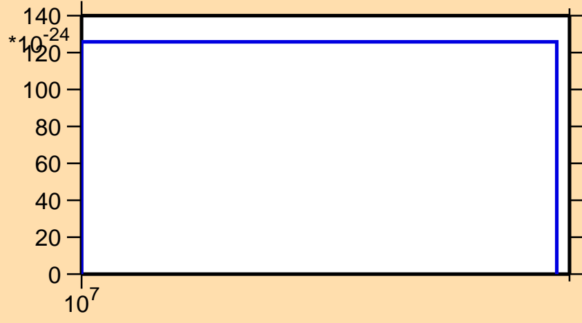
\sigma vs. E for ^{181}\text{Au} (mt 42)
