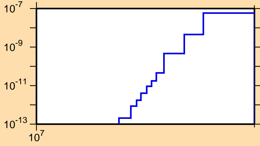
\sigma vs. E for ^{182}\text{Au}(n,\text{pt})
