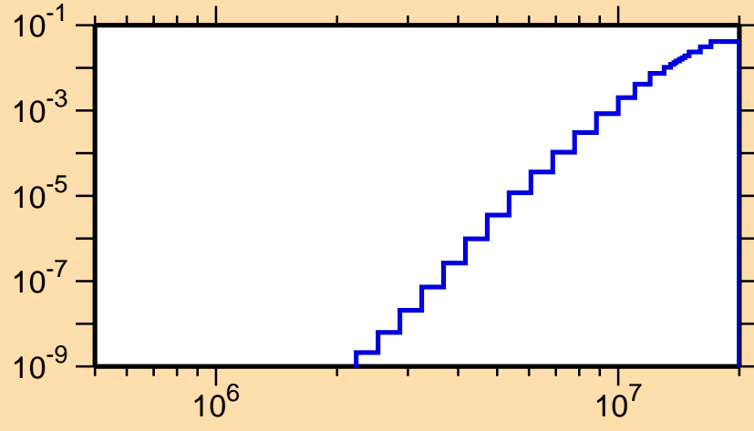
\sigma vs. E for ^{182}\text{Au}(n,n\alpha)
