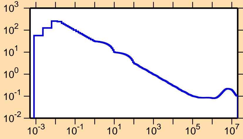
\sigma vs. E for ^{182}\text{Au}(n,p)
