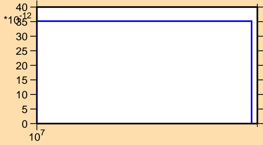
\sigma vs. E for ^{182}\text{Au} (mt 34)
