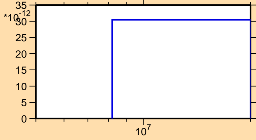
\sigma vs. E for ^{182}\text{Au}(\text{mt } 34)
