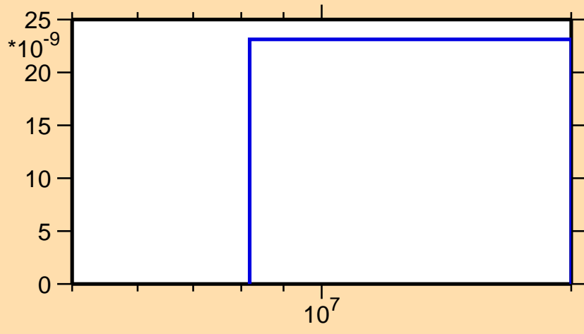
\sigma vs. E for ^{182}\text{Au}(n,3n)
