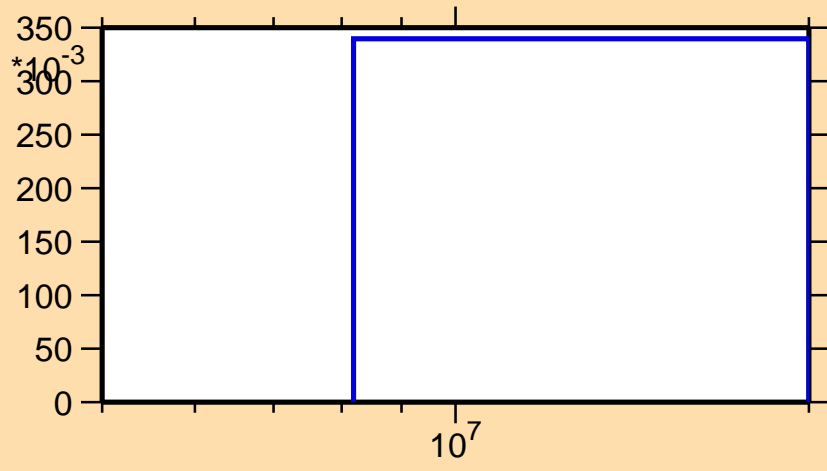
\sigma vs. E for ^{182}\text{Au}(n,2n)
