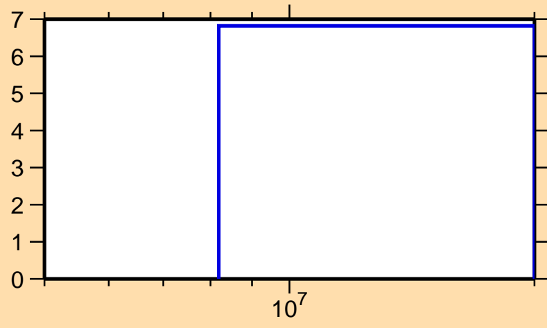
\Delta\sigma/\sigma vs. E for ^{182}\text{Au}(n,\text{tot.})
