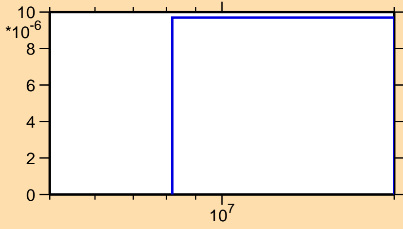
\sigma vs. E for ^{182}\text{Au}(n,2n\alpha)
