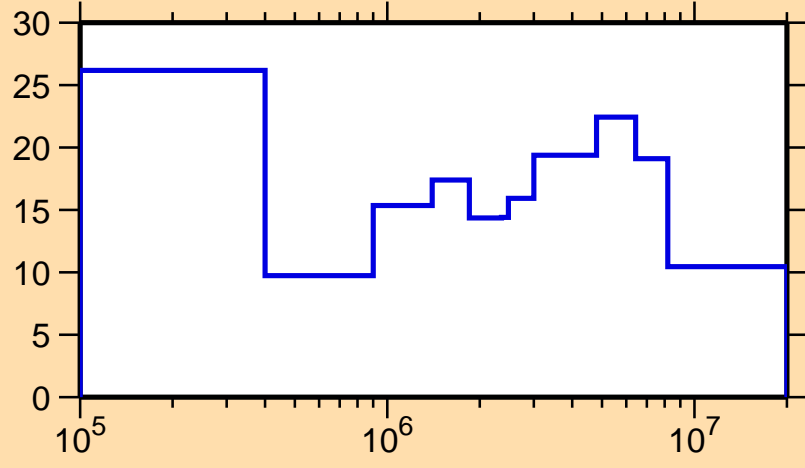
\Delta\sigma/\sigma vs. E for ^{182}\text{Au}(n,\text{el.})
