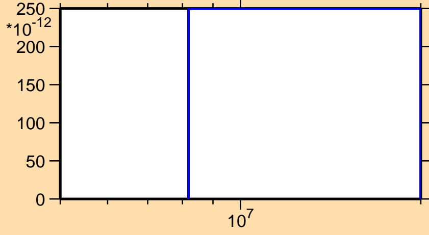
\sigma vs. E for ^{182}\text{Au}(n,nt)
