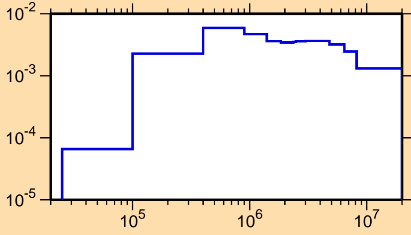
\sigma vs. E for ^{182}\text{Au}(n,n_2)
