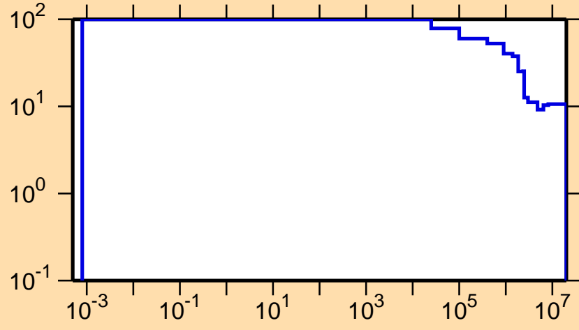
\Delta\sigma/\sigma vs. E for ^{182}\text{Au}(n,\text{nonel.})
