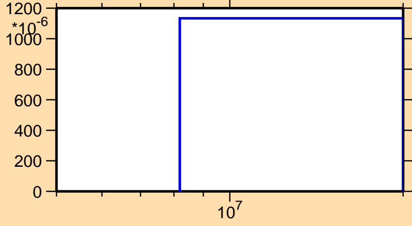
\sigma vs. E for ^{182}\text{Au}(n,2np)
