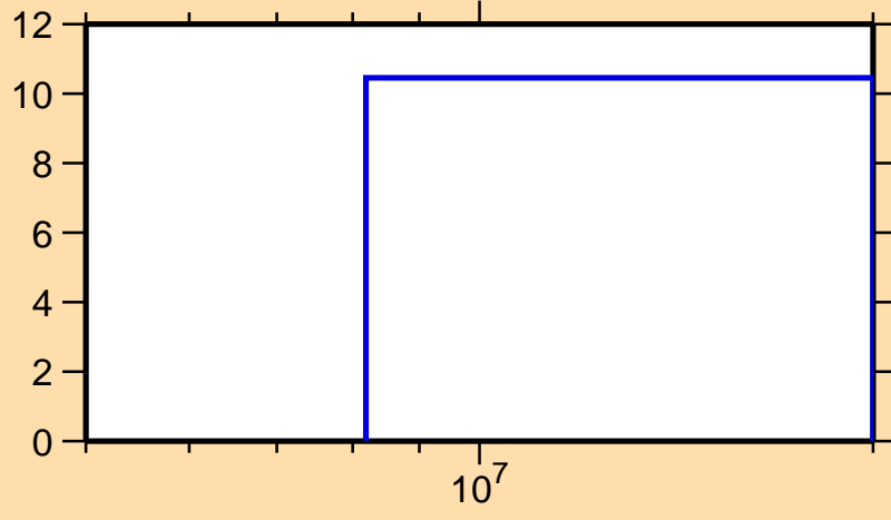
\Delta\sigma/\sigma vs. E for ^{182}\text{Au}(n,\text{el.})
