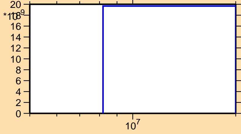
\sigma vs. E for ^{182}\text{Au}(n,\text{pd})
