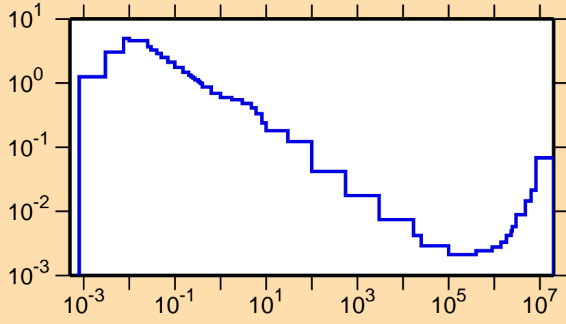
\sigma vs. E for ^{182}\text{Au}(n,\alpha)
