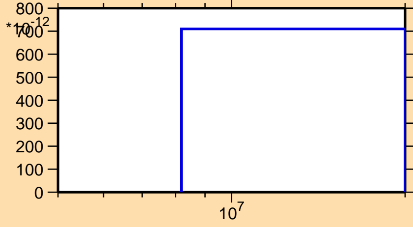
\sigma vs. E for ^{182}\text{Au}(n,\text{pt})
