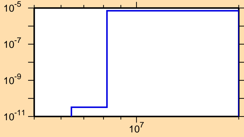
\sigma vs. E for ^{182}\text{Au}(n,\text{He3})
