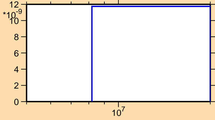
\sigma vs. E for ^{182}\text{Au}(\text{mt117})
