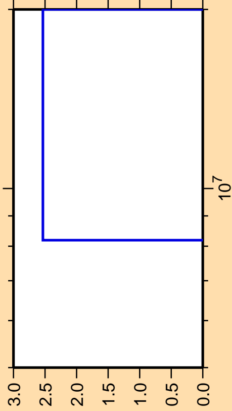
\Delta\sigma/\sigma vs. E for ^{182}\text{Au}(n,3n\alpha)
