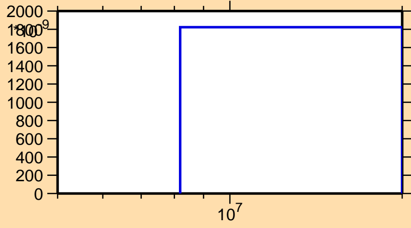
\sigma vs. E for ^{182}\text{Au}(n,nd)
