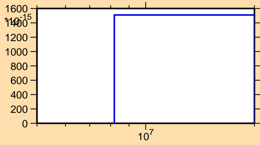
\sigma vs. E for ^{182}\text{Au}(n,3n\alpha)
