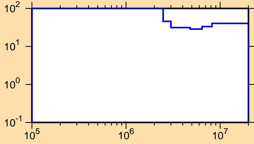
\Delta\sigma/\sigma vs. E for ^{182}\text{Au}(n,n\text{cont.})
