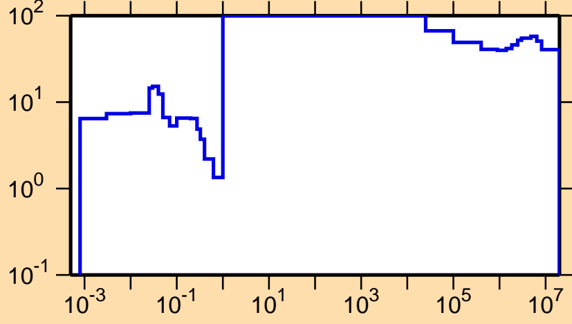
\Delta\sigma/\sigma vs. E for ^{182}\text{Au}(n,\gamma)
