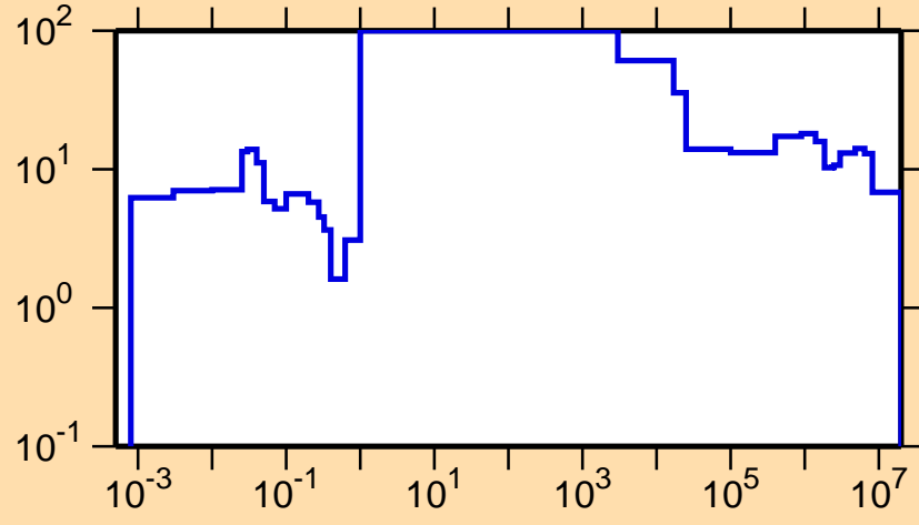
\Delta\sigma/\sigma vs. E for ^{182}\text{Au}(n,\text{tot.})
