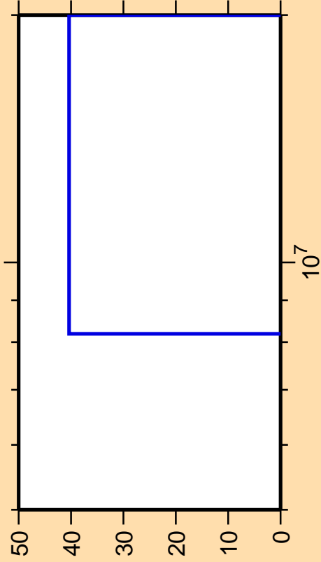
\Delta\sigma/\sigma vs. E for ^{182}\text{Au}(n,n\text{cont.})
