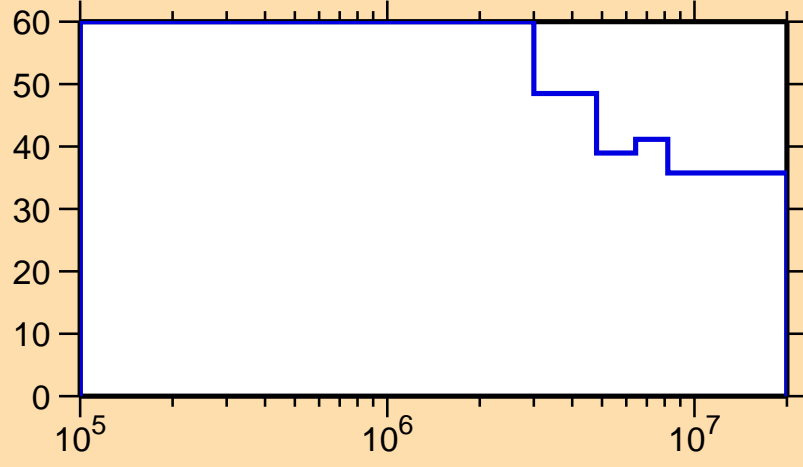
\Delta\sigma/\sigma vs. E for ^{182}\text{Au}(n,n_1)
