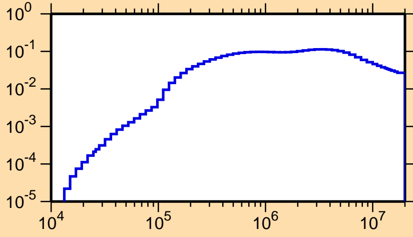
\sigma vs. E for ^{183}\text{Au}(n,n_1)
