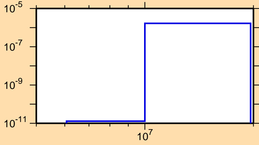
\sigma vs. E for ^{183}\text{Au}(\text{mt } 45)
