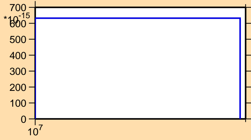
\sigma vs. E for ^{183}\text{Au} (mt 34)
