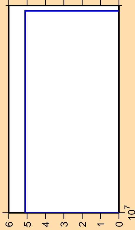
\Delta\sigma/\sigma vs. E for ^{183}\text{Au} (mt 34)
