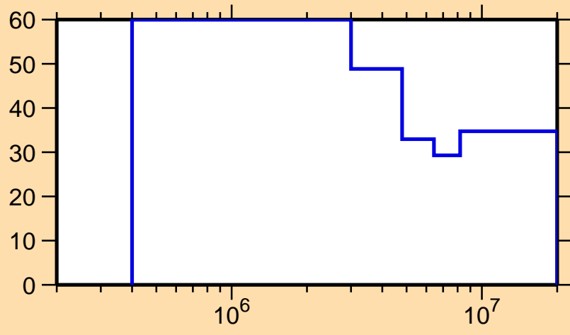
\Delta\sigma/\sigma vs. E for ^{183}\text{Au}(n,n\text{cont.})
