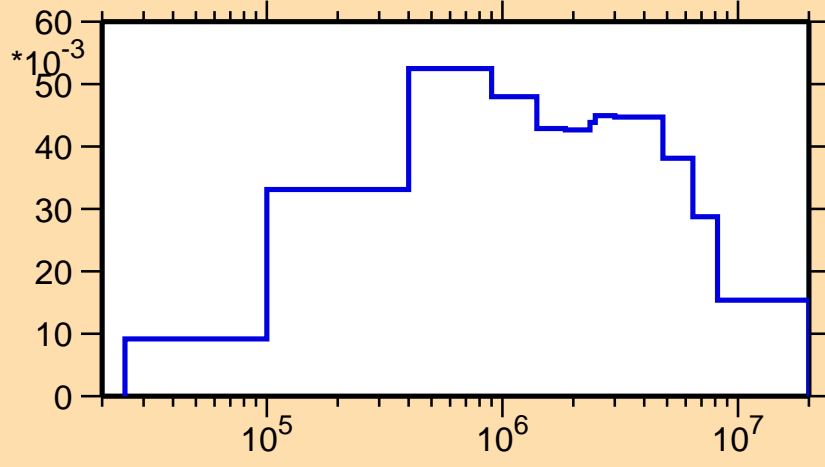
\sigma vs. E for ^{183}\text{Au}(n,n_2)
