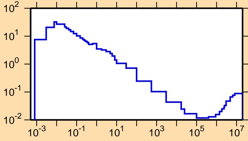
\sigma vs. E for ^{184}\text{Au}(n,p)
