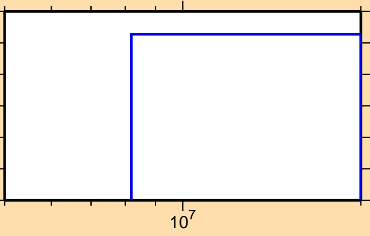
\sigma vs. E for ^{184}\text{Au}(n,nt)
