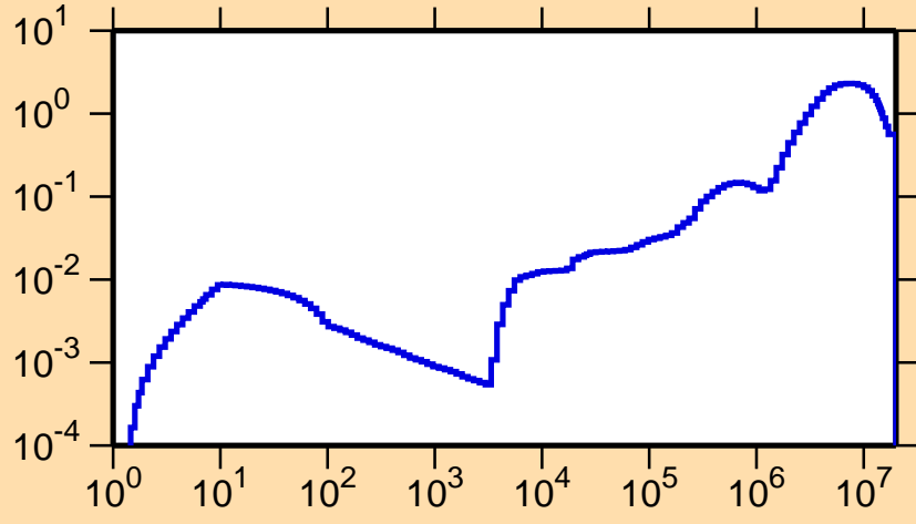
\sigma vs. E for ^{184}\text{Au}(n,\text{inel.})
