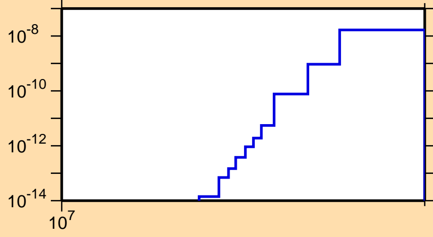
\sigma vs. E for ^{184}\text{Au}(n,pt)
