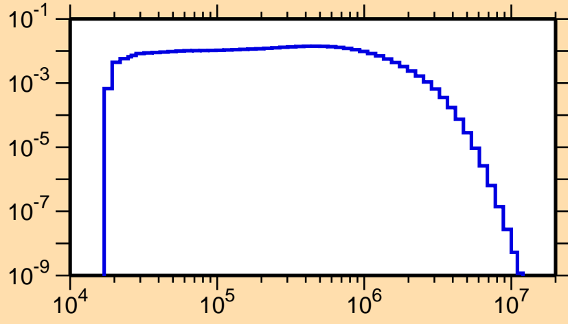
\sigma vs. E for ^{184}\text{Au}(n,n_4)
