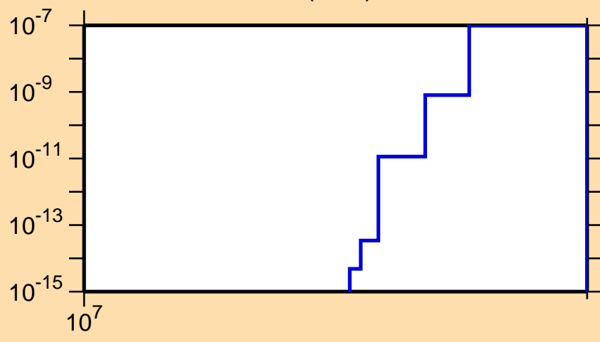
\sigma vs. E for ^{184}\text{Au}(n,nt)
