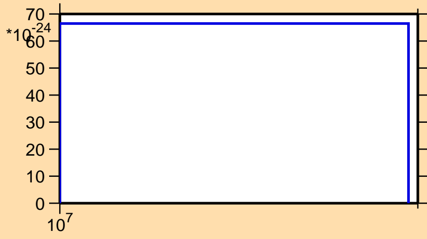
\sigma vs. E for ^{184}\text{Au}(\text{mt } 42)
