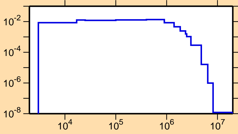
\sigma vs. E for ^{184}\text{Au}(n,n_2)
