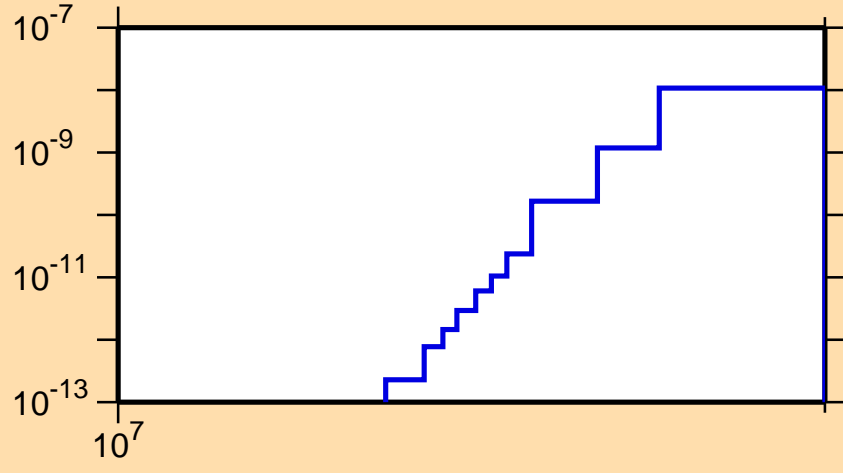
\sigma vs. E for ^{186}\text{Au}(n,\text{pd})
