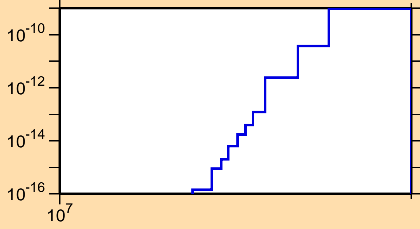
\sigma vs. E for ^{186}\text{Au}(n,pt)
