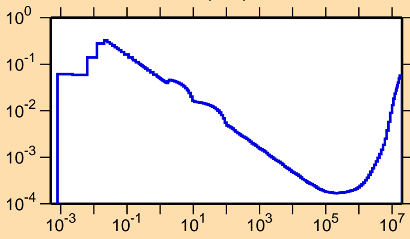
\sigma vs. E for ^{186}\text{Au}(n,\alpha)
