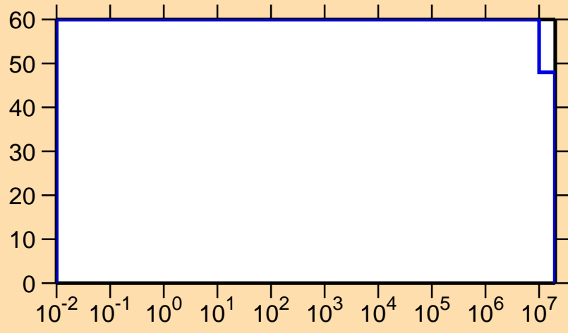
\Delta\sigma/\sigma vs. E for ^{186}\text{Au}(n,p)
