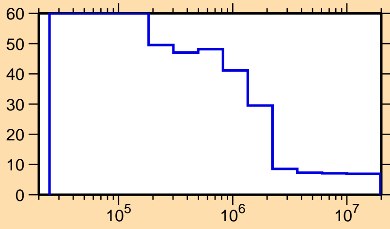
\Delta\sigma/\sigma vs. E for ^{186}\text{Au}(n,\text{nonel.})
