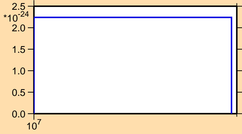
\sigma vs. E for ^{186}\text{Au} (mt 42)
