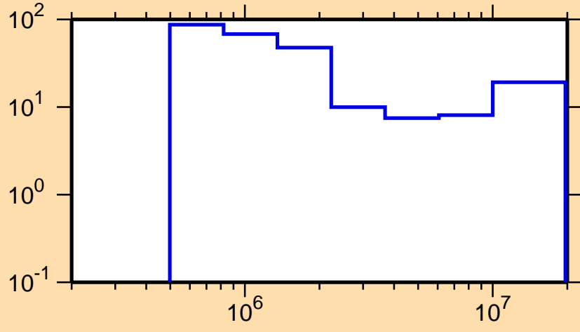
\Delta\sigma/\sigma vs. E for ^{186}\text{Au}(n,n\text{cont.})
