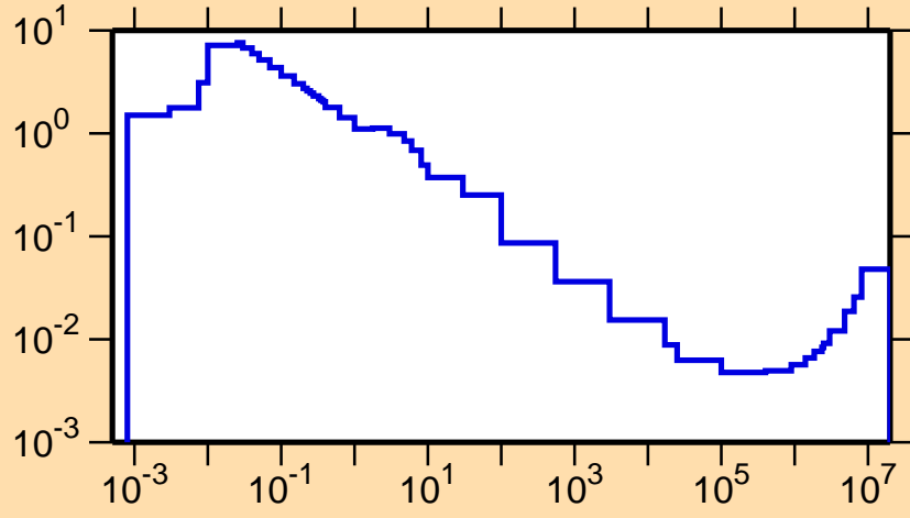
\sigma vs. E for ^{186}\text{Au}(n,p)
