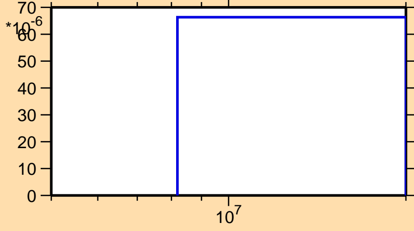
\sigma vs. E for ^{186}\text{Au}(n,2np)
