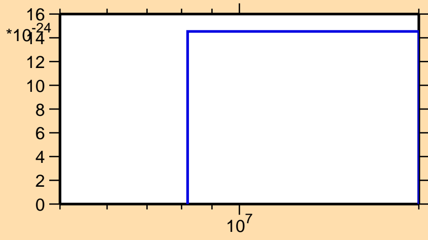
\sigma vs. E for ^{186}\text{Au}(\text{mt } 42)
