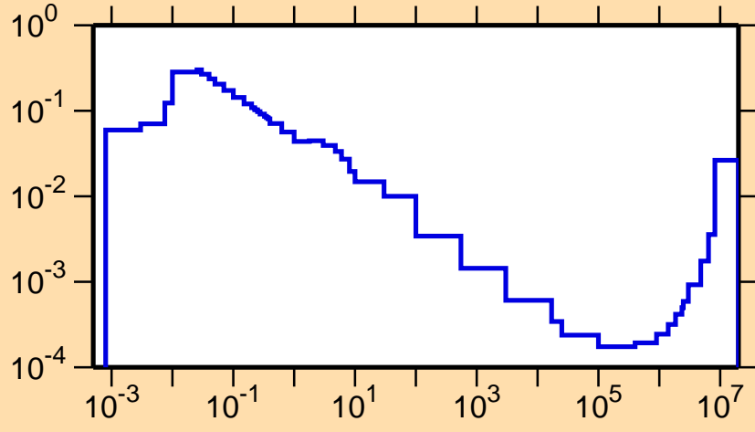
\sigma vs. E for ^{186}\text{Au}(n,\alpha)
